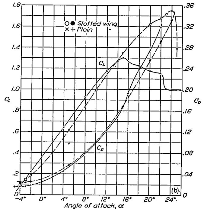
FIGURE 4.—Characteristics of Clark Y wing with best fixed slot
