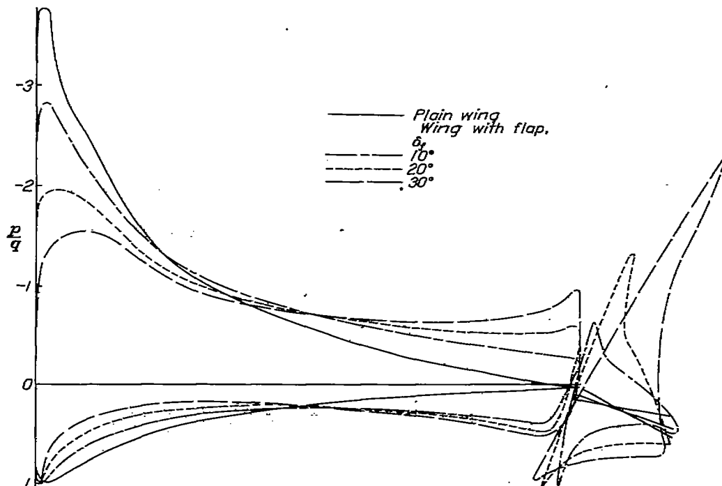
Figure 33.- Comparison of the pressure distribution over an N.A.C.A. 23012 wing with a 0.20c_w external-airfoil flap with that over the plain wing at the same lift, c_n, 1.165 , (reference 15)
