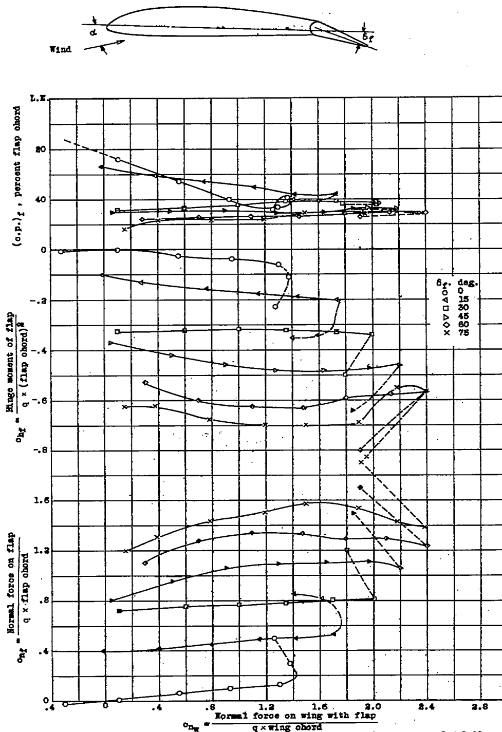
Figure 12. Normal-force and hinge-moment coefficients and centers of pressure of a 0.80 c_w plain flap on an N.A.C.A. 23013 wing. Flap deflections from 0° to 75°. (reference ?)
