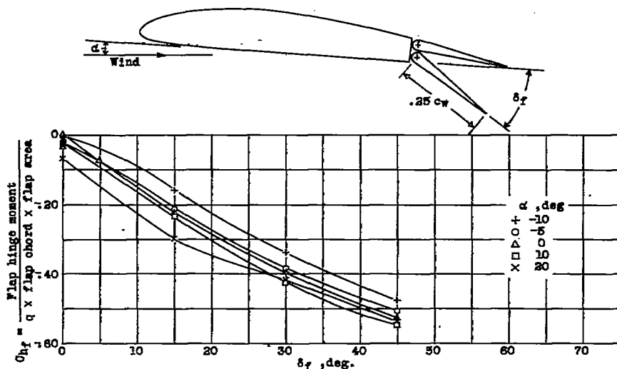
Figure 18. Hinge-moment coefficients of a 0.25c_w split flap on a Clark Y wing (reference 9).
