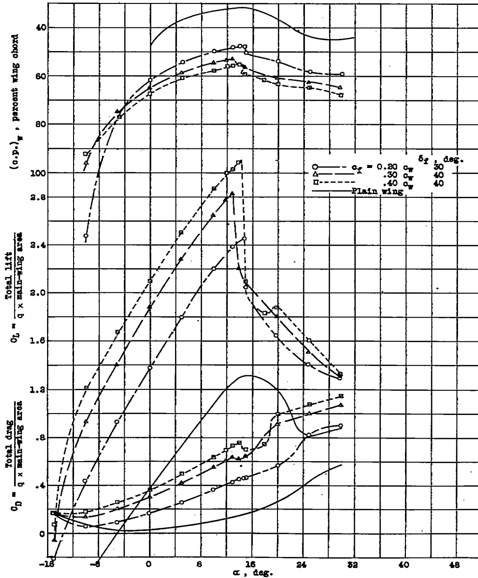
Figure 28.- Lift and drag coefficients and centers of pressure of a plain Clark Y wing and of a Clark Y wing with three sizes of Fowler flap, (reference 12).
