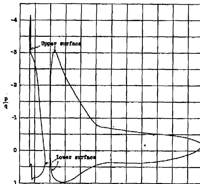
Figure 2. Pressure-distribution diagram for slotted R.A.F. 31 wing, \alpha = 25^\circ (reference 1).
