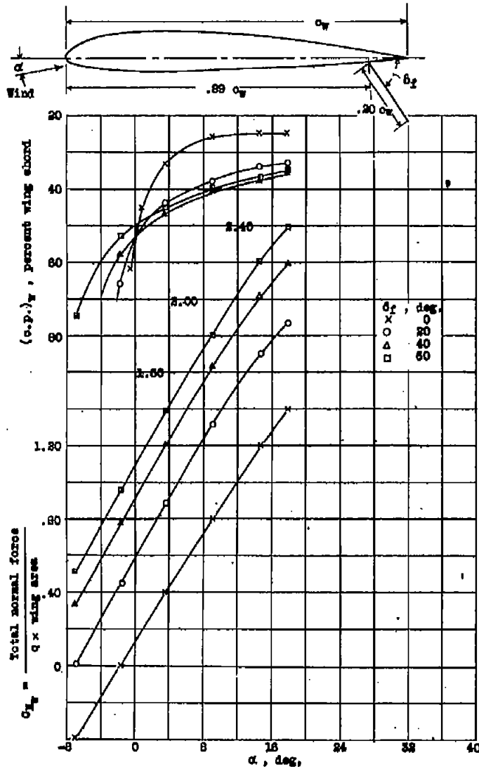
Figure 23.- Normal-force coefficients and centers of pressure of an N.A.C.A. 2212 wing with a 0.20 c_w split flap (lap) at 0.89 c_w , (reference 10).
