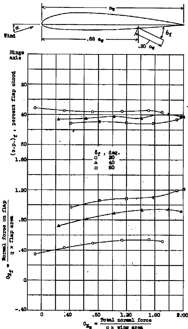
Figure 20.- Normal-force coefficients and centers of pressure of a 0.20 c_w split flap at 0.68 c_w on an N.A.C.A. 2212 wing, (reference 10).
