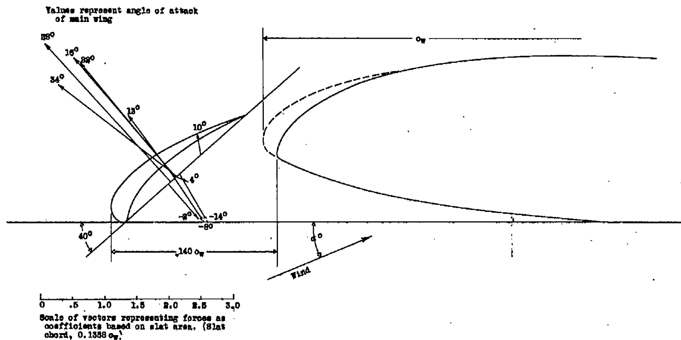
Figure 5. Vector diagram representing forces on slat with slot fully open (reference 1)
