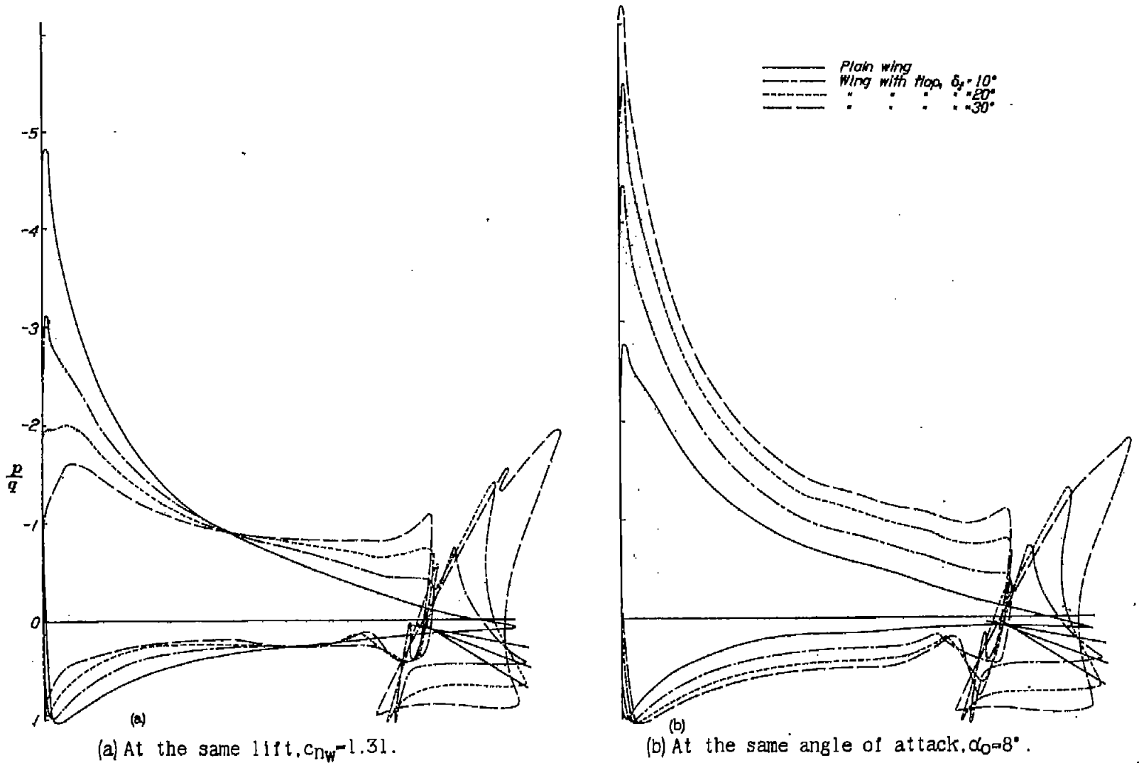
Figure 26.- Comparison of the pressure distribution on an N.A.C.A. 23012 wing and a 0.2566 c_w slotted flap with that on the plain wing.
