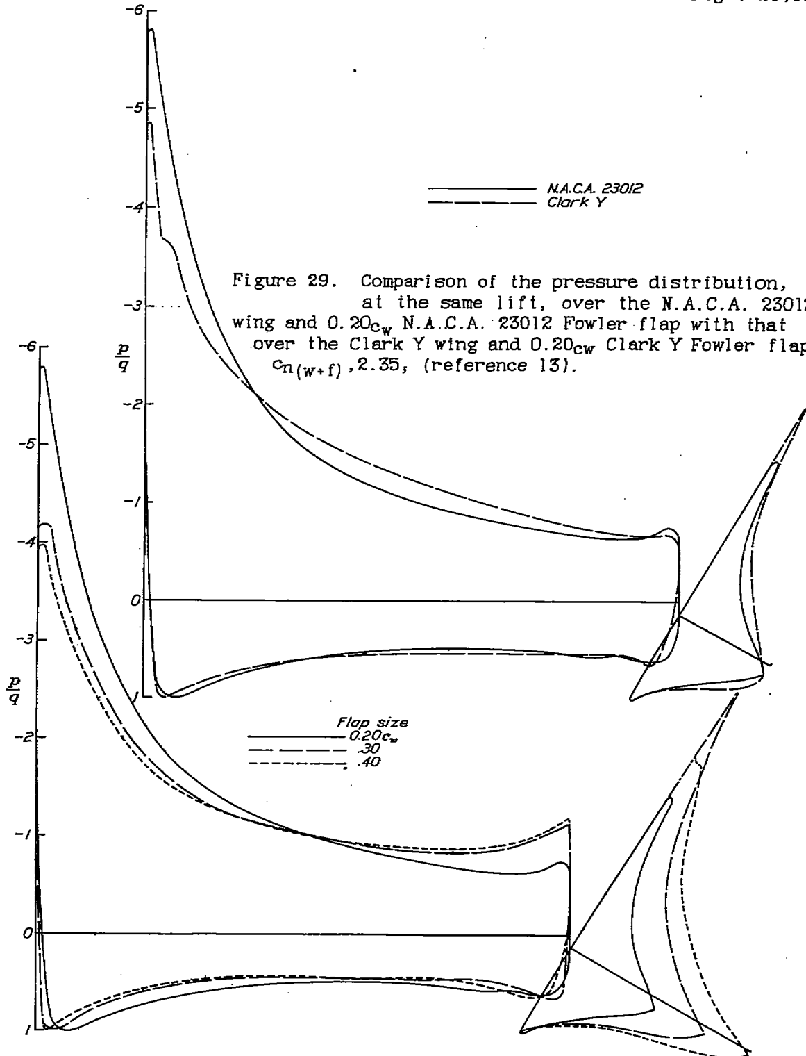
Figure 30. - Comparison of the pressure distribution, at the same lift, over the N.A.C.A. 23012 wing with 0.20c w , 0.30c w & 0.40c w NACA 23012 Fowler flaps, C n(w+f) , 2.35, (reference 13).
