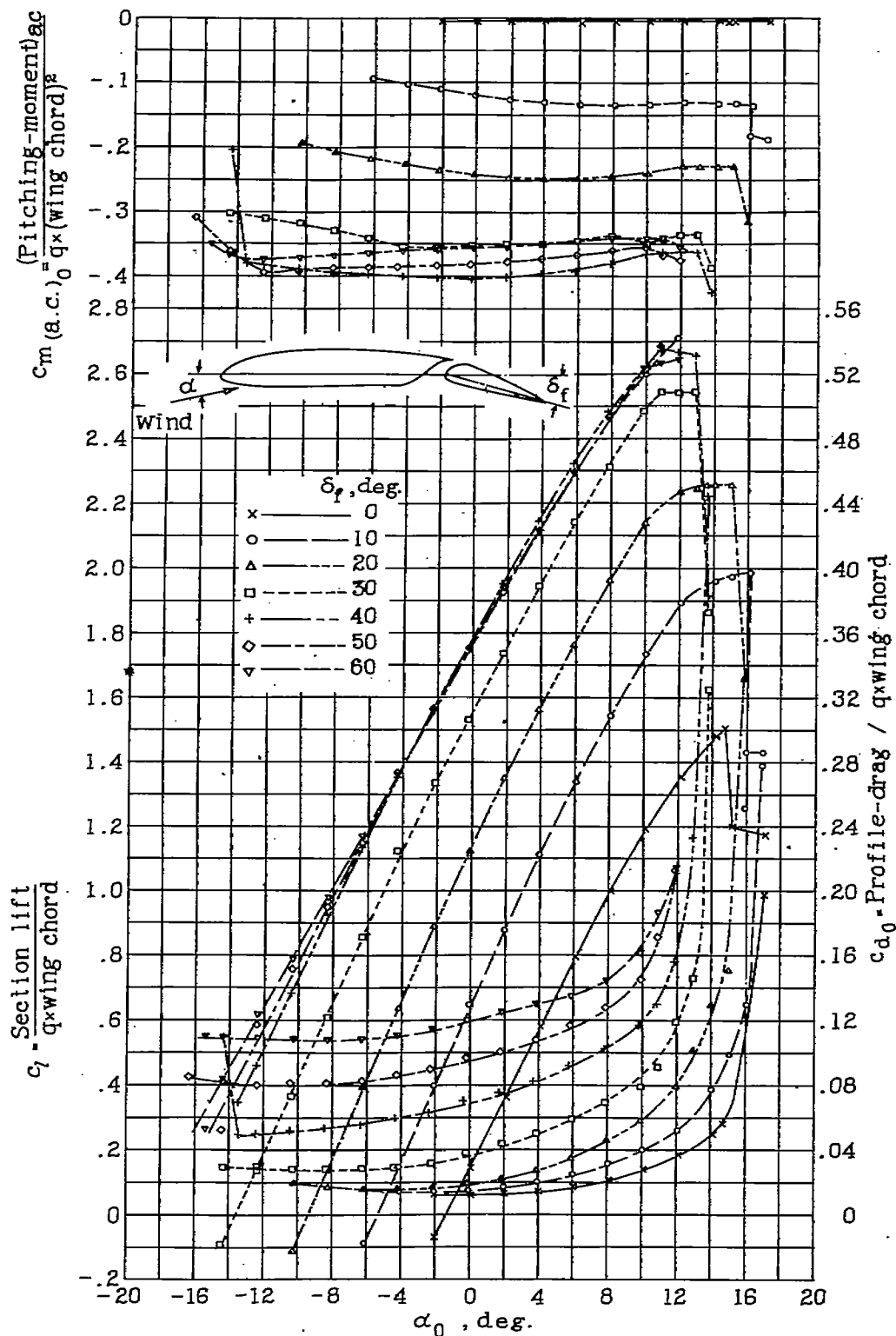
Figure 25.- Section lift, drag, and pitching-moment coefficients of an N.A.C.A. 23012 wing with a 0.2566 c_w slotted flap. (reference 11)
