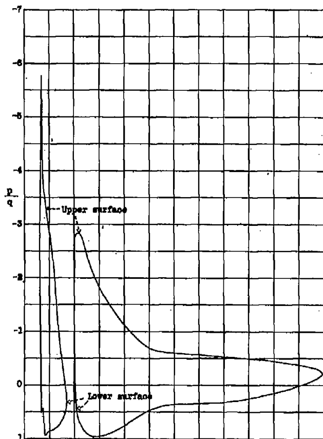
Figure 5.- Pressure-distribution diagram for slotted R.A.F. 31 wing, \alpha = 8^\circ (reference 1).
