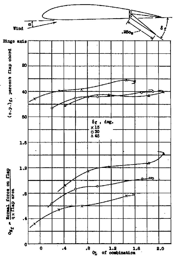
Figure 16.- Normal-force coefficients and centers of pressure of a 0.25c_w split flap on a Clark Y wing, (reference 9).
