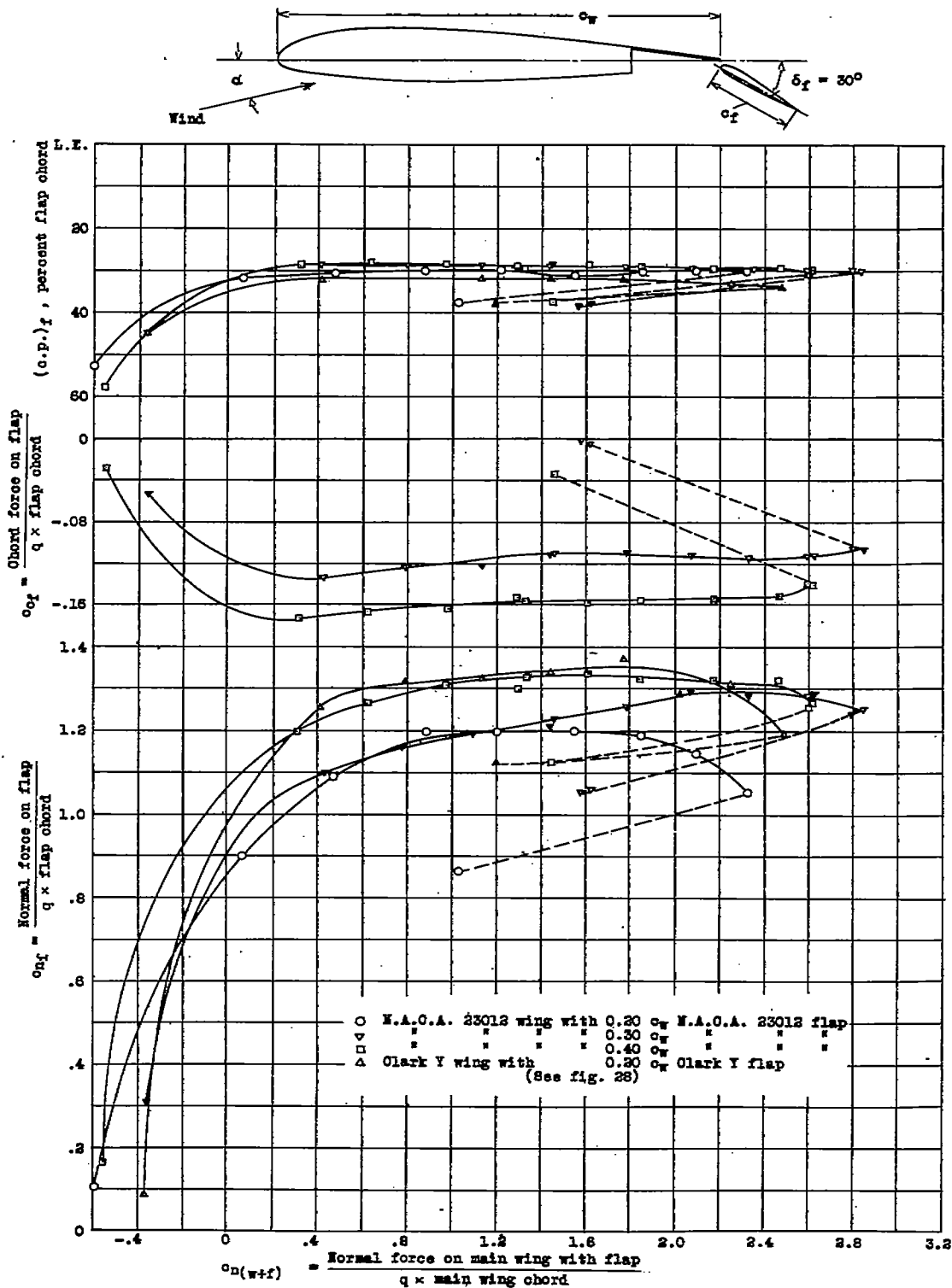
Figure 31.- Normal-force and chord-force coefficients and centers of pressure of Fowler flap on Clark Y and N.A.C.A. 23012 wings, (reference 13).
