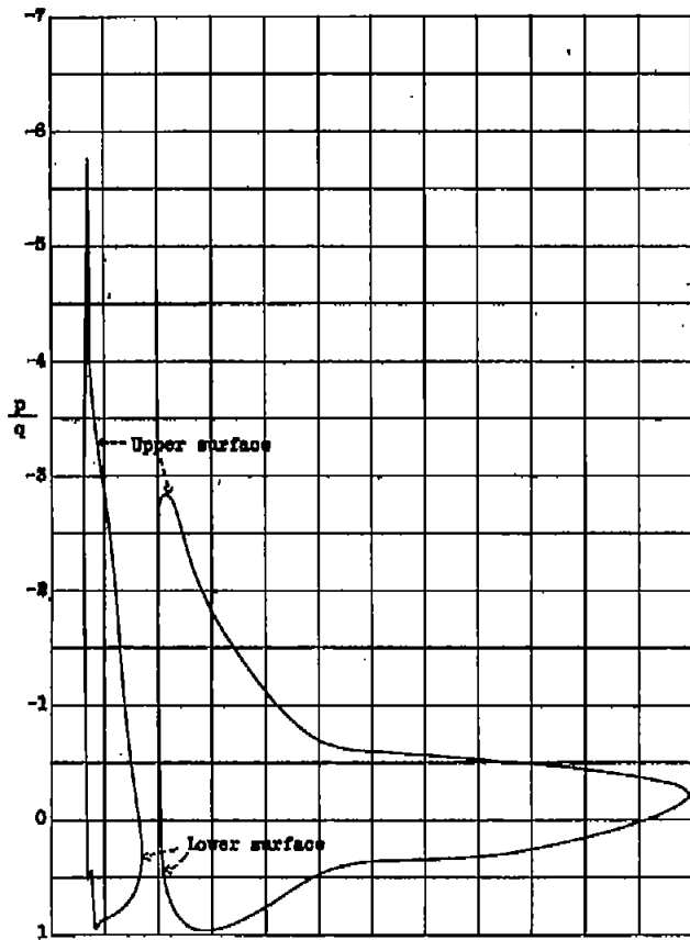
Figure 3.- Pressure-distribution diagram for slotted R.A.F. 31 wing, \alpha = 31^\circ (reference 1).
