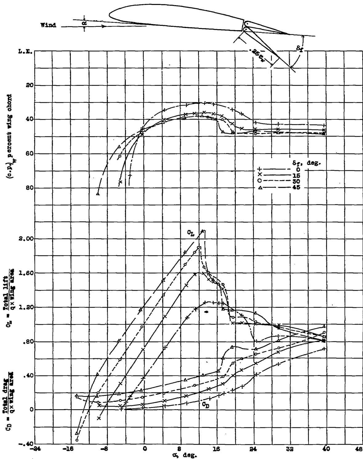
Figure 14.- Lift and drag coefficients and center of pressure of a Clark Y wing with a 0.25c_w split flap (reference 9).
