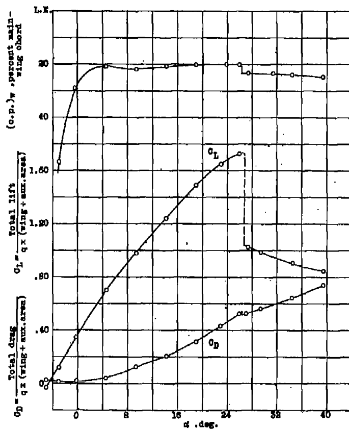
Figure 6.- Lift and drag coefficients and centers of pressure of a Clark Y wing with an N.A.C.A. 23 auxiliary airfoil; \delta_{aux}, 0^\circ (reference 4).
