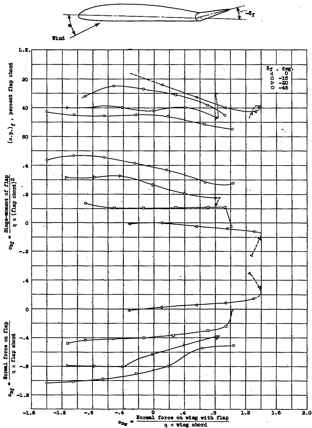
Figure 11.- Normal-force and hinge-moment coefficients, and centers of pressure of a 0.80 c_w plain flap on an N.A.C.A. 23012 wing. Flap deflections from 0^\circ to -45^\circ , (reference 7).
