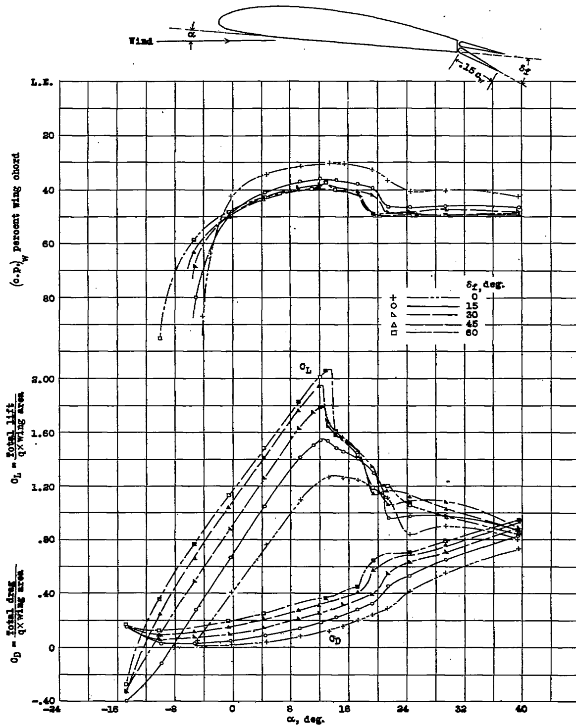
Figure 13.— Lift and drag coefficients and center of pressure of a Clark Y wing with a 0.15c_w split flap (reference 9).
