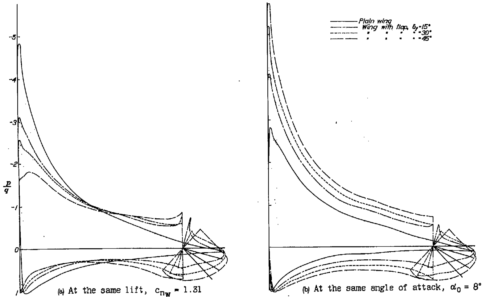
Figure 10.- Comparison of the pressure distribution on an N.A.C.A. 23012 wing and a 0.20 c_w plain flap with that on the plain wing, (reference 7).
