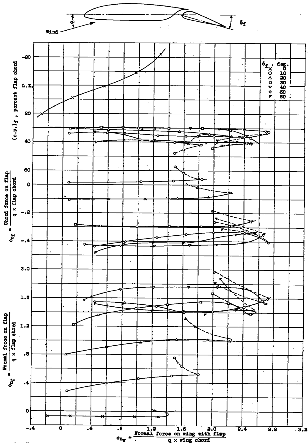
Figure 27.- Normal-force and chord-force coefficients and centers of pressure of a 0.2566 c_w slotted flap on a N.A.C.A. 23012 wing, (reference 7).
