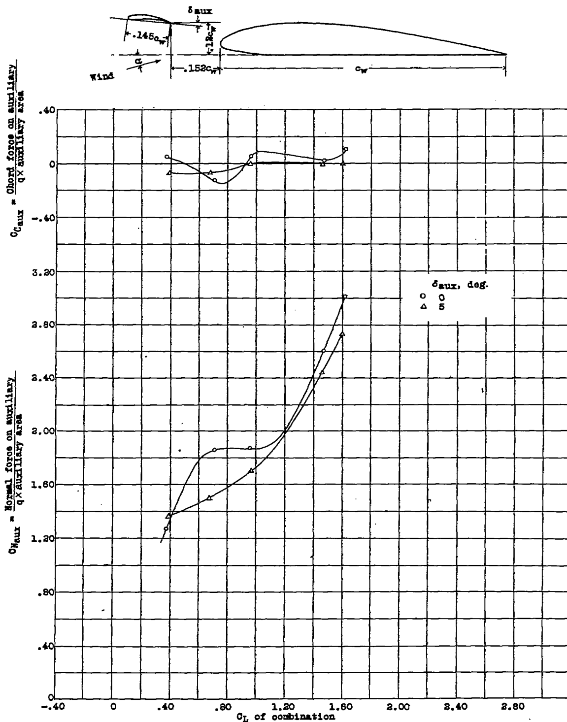
Figure 7.- Normal and chord-force coefficients of N.A.C.A. 23 auxiliary airfoil ahead of a Clark Y wing (reference 5).
