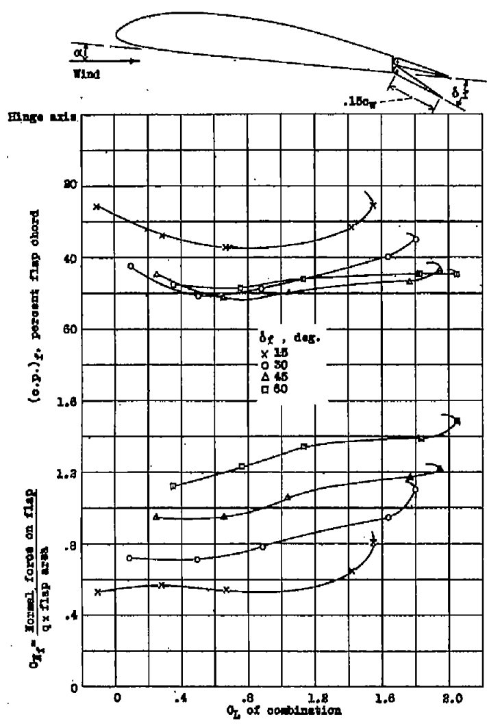
Figure 15.- Normal-force coefficients and centers of pressure of a 0.15c_w split flap on a Clark Y wing, (reference 9).
