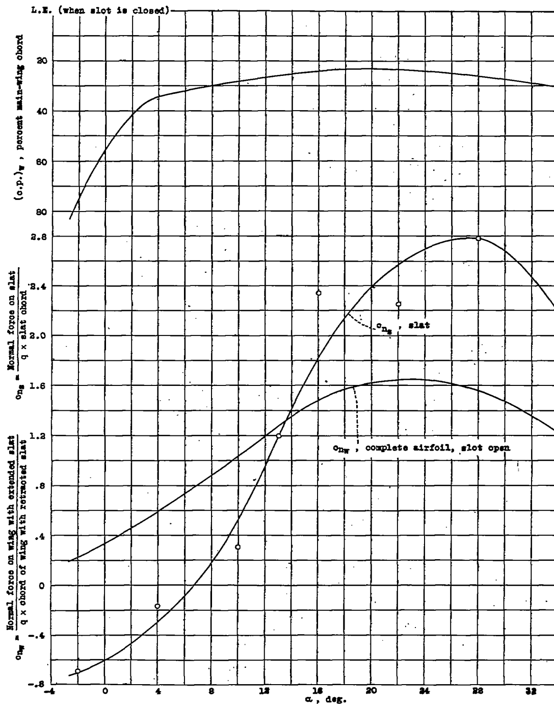
Figure 4.- Normal-force coefficients and centers of pressure of a slotted R.A.F. 31 wing, and normal-force coefficients of the slat, (reference 1).
