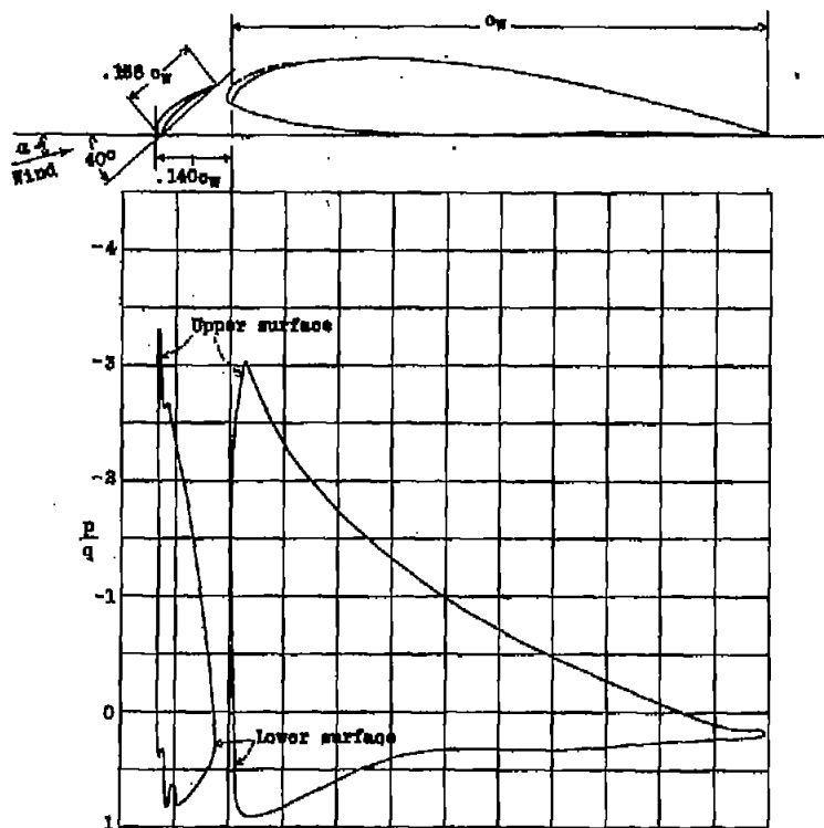
Figure 1.- Pressure-distribution diagram for slotted R.A.F. 31 wing, \alpha = 16^\circ (reference 1).
