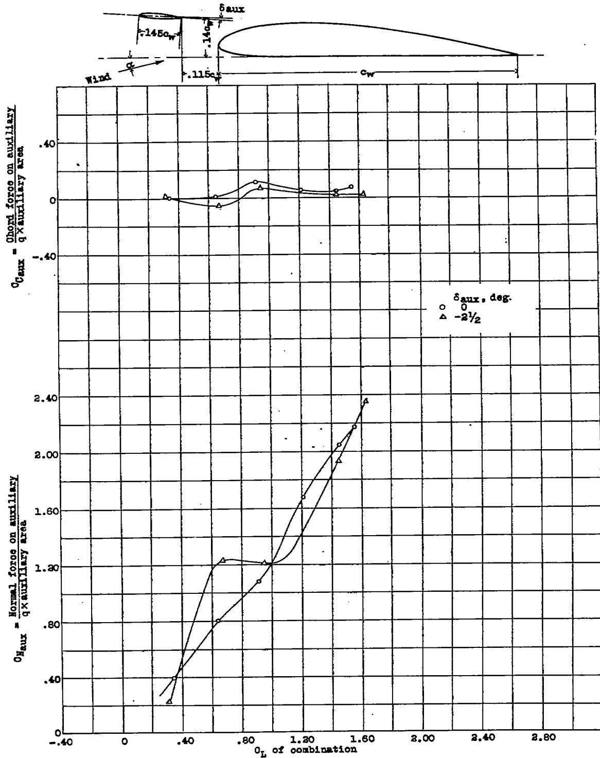
Figure 8.-- Normal and chord-force coefficients of N.A.C.A. 0012 auxiliary airfoil ahead of a Clark Y wing (reference 5).
