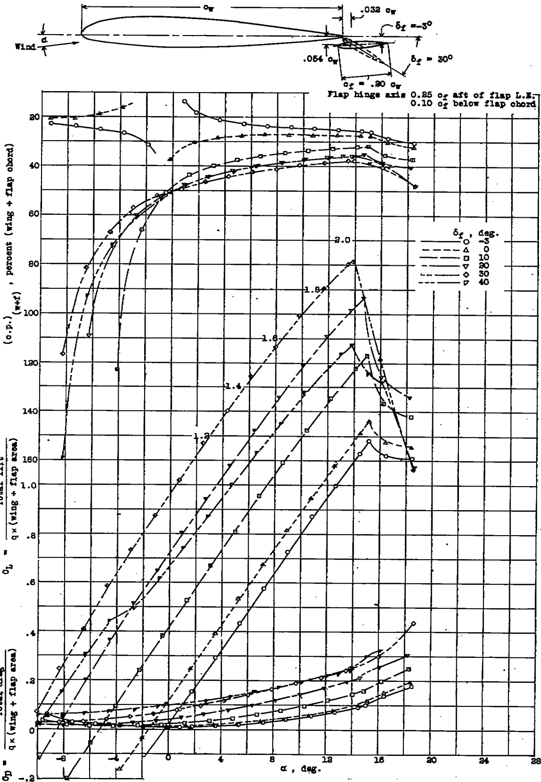
Figure 32. - Lift and drag coefficients and centers of pressure of an N.A.C.A. 23012 wing with a 0.20 c_w N.A.C.A. 23012 external-airfoil flap, (reference 14).
