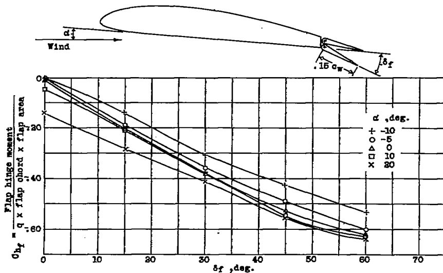
Figure 17. Hinge-moment coefficients of a 0.15c_w split flap on a Clark Y wing (reference 9).
