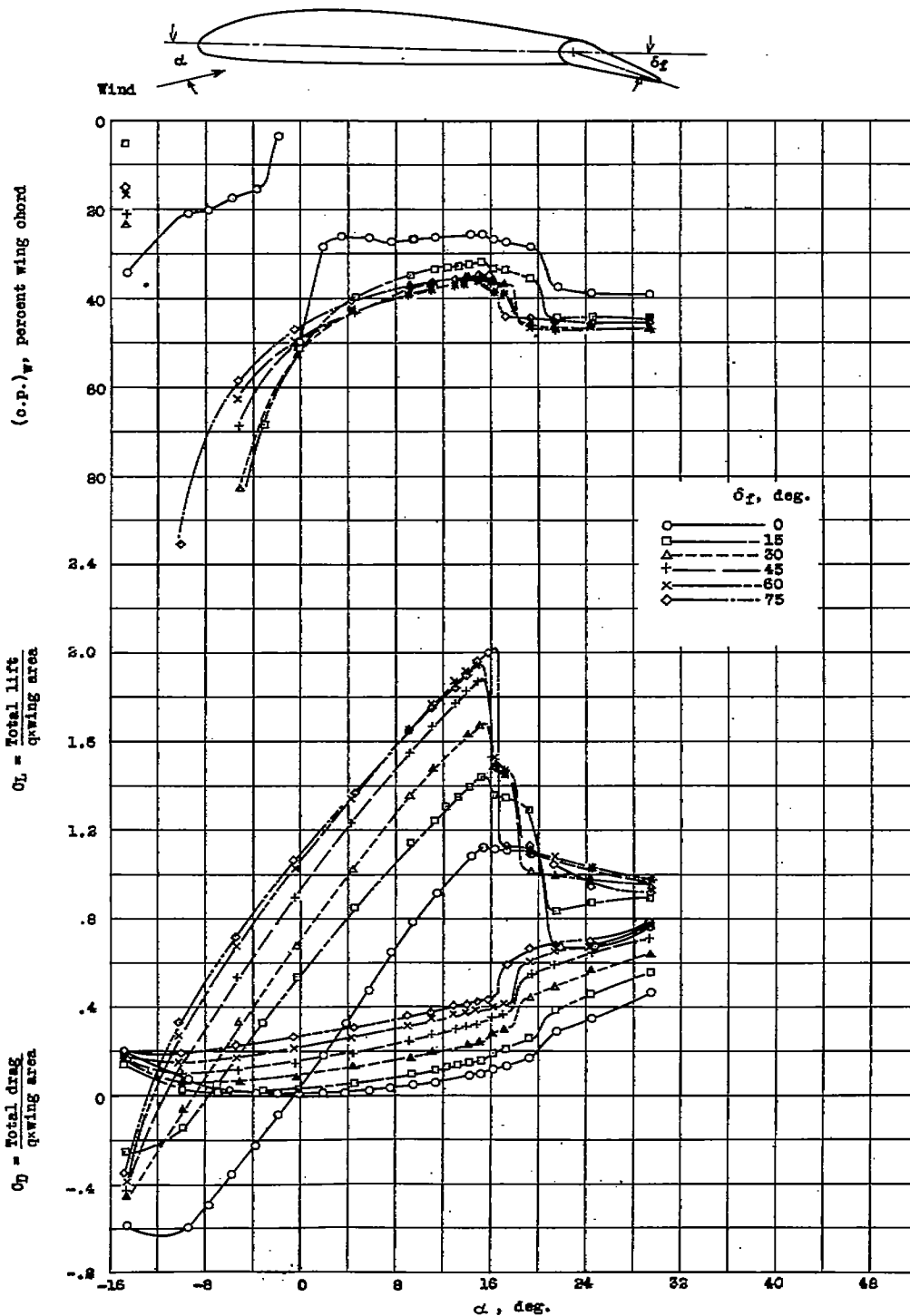
Figure 9.- Lift and drag coefficients and centers of pressure of an N.A.C.A. 23012 wing with a 0.30 c_w plain flap, (reference 6).
