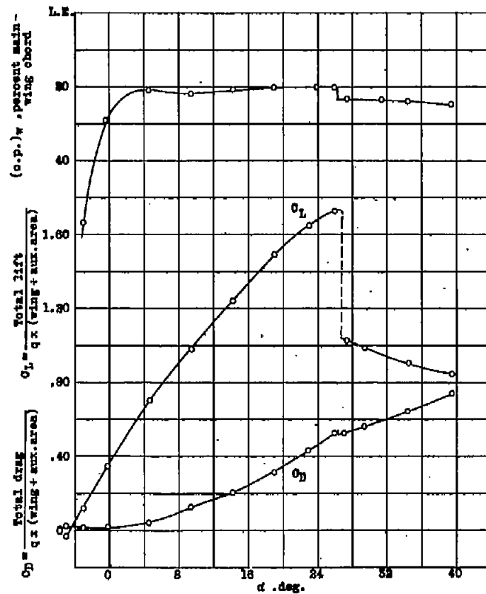
Figure 5.- Lift and drag coefficients and centers of pressure of a Clark Y wing with an N.A.C.A. 23 auxiliary airfoil, \delta_{aux} = 0^\circ (reference 4).
