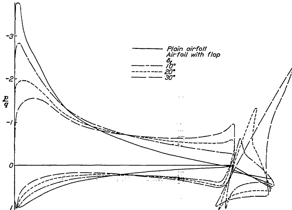
FIGURE 10.—Comparison of the pressure distribution on an N. A. C. A. 23012 airfoil with a 0.20c_w external-airfoil flap with that on the plain airfoil at the same lift, c_L=1.165 .
