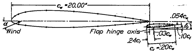
FIGURE 1.—Cross section of model showing orifice locations used in pressure-distribution tests. N. A. C. A. 23012 airfoil with 0.20c_w 23012 external-airfoil flap.
