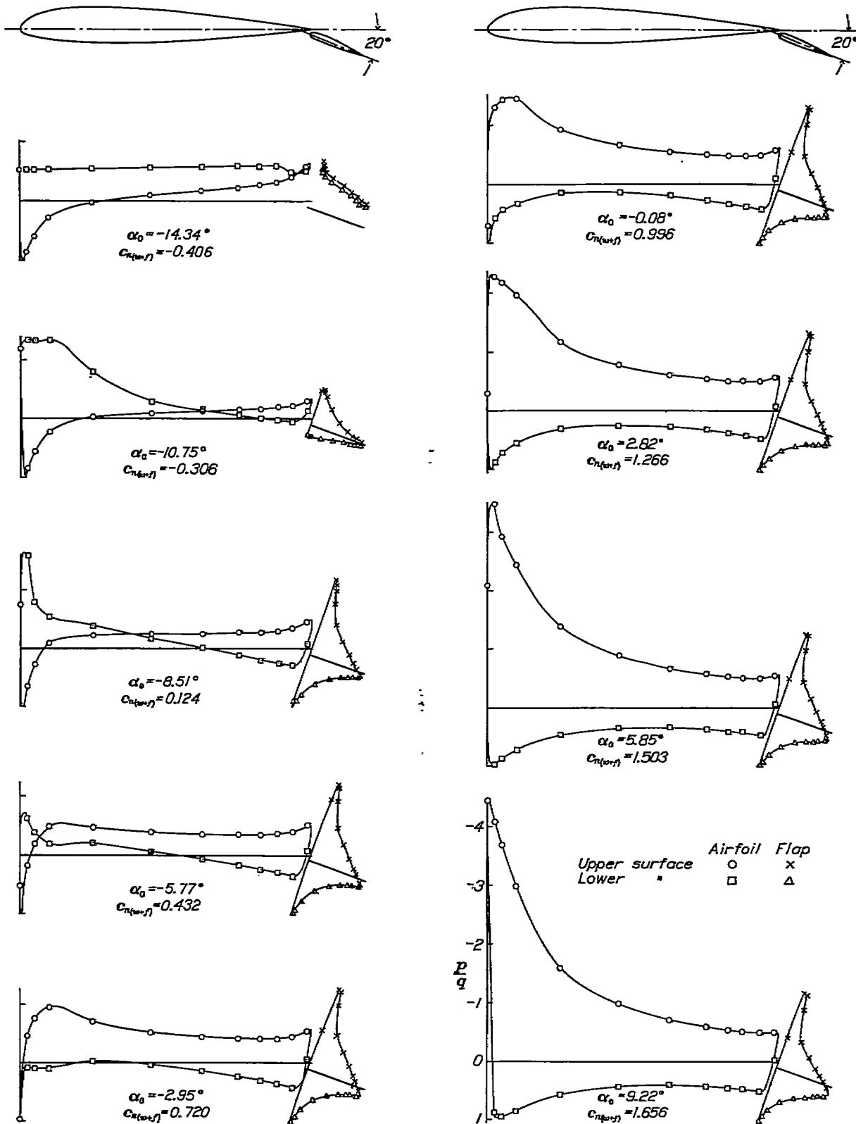
FIGURE 7.—Pressure distribution on the N. A. C. A. 23012 airfoil with N. A. C. A. 28012 external-airfoil flap at various angles of attack. Flap deflected 20^\circ .
