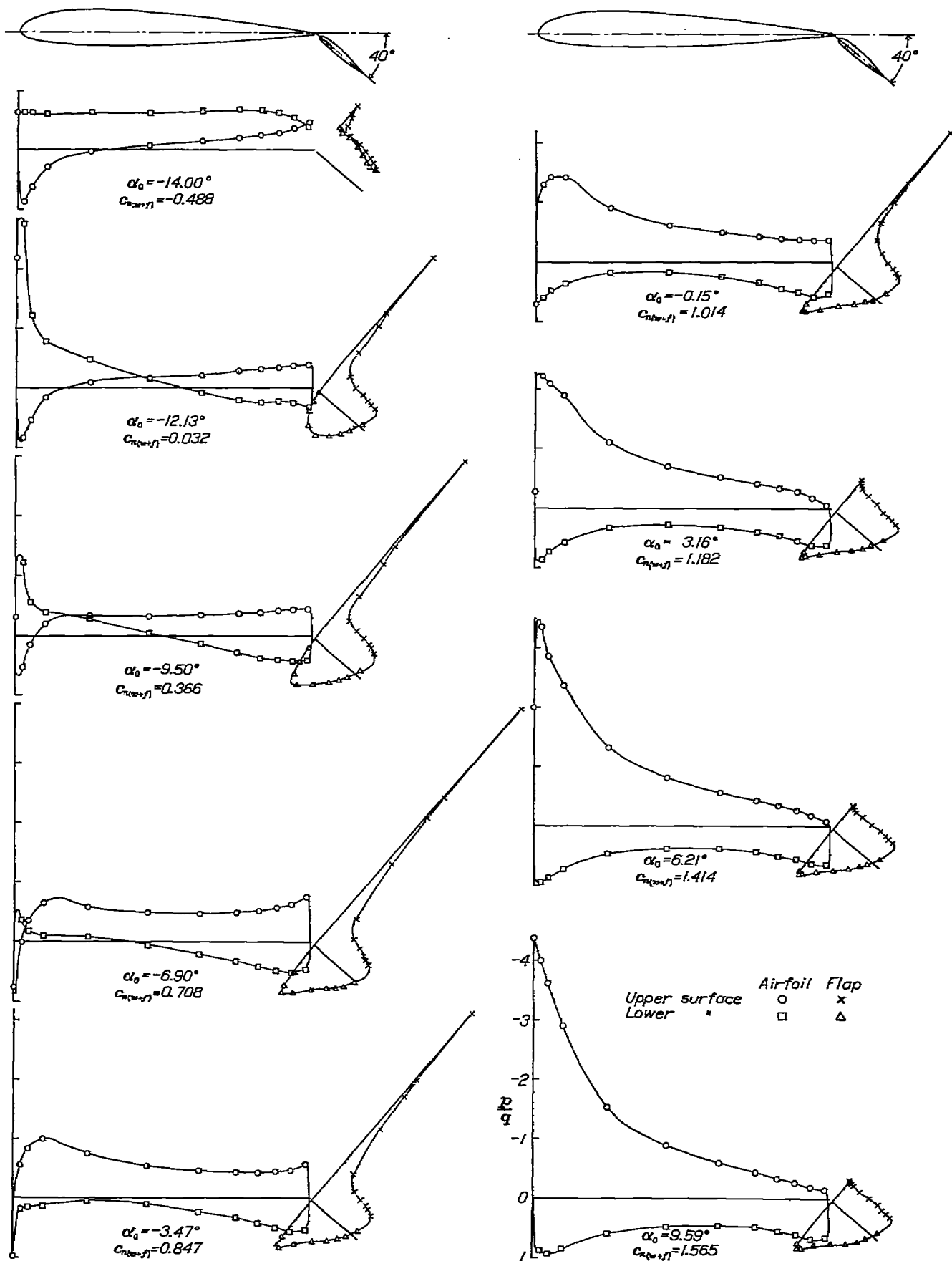
FIGURE 9.—Pressure distribution on the N. A. C. A. 23012 airfoil with N. A. G. A. 23012 external-airfoil flap at various angles of attack. Flap deflected 40°.
