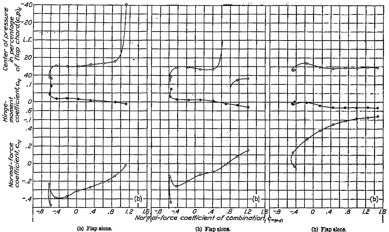
FIGURE 13.—Section characteristics of the N. A. C. A. 23012 airfoil with a 0.20c N. A. C. A. 23012 external-airfoil flap set at -3^\circ .
