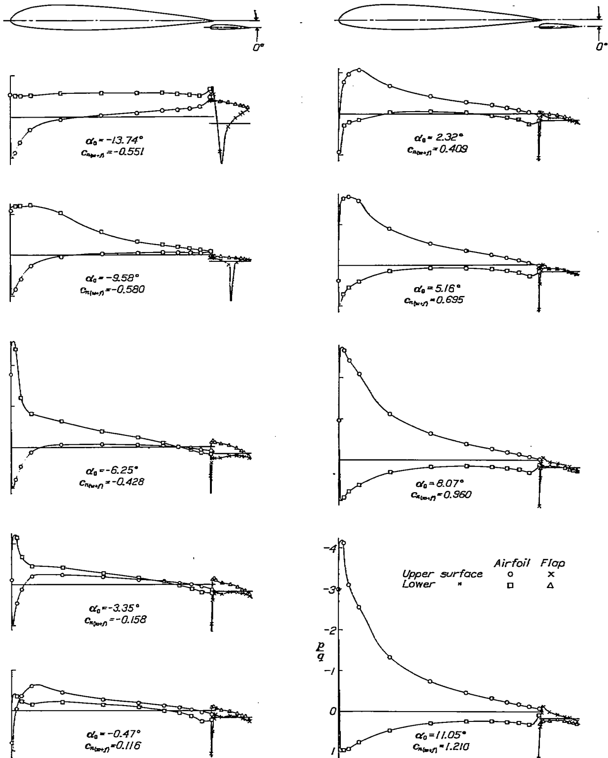
FIGURE 5.—Pressure distribution on the N. A. C. A. 23012 airfoil with N. A. C. A. 23012 external-airfoil flap at various angles of attack. Flap deflected 0°.
