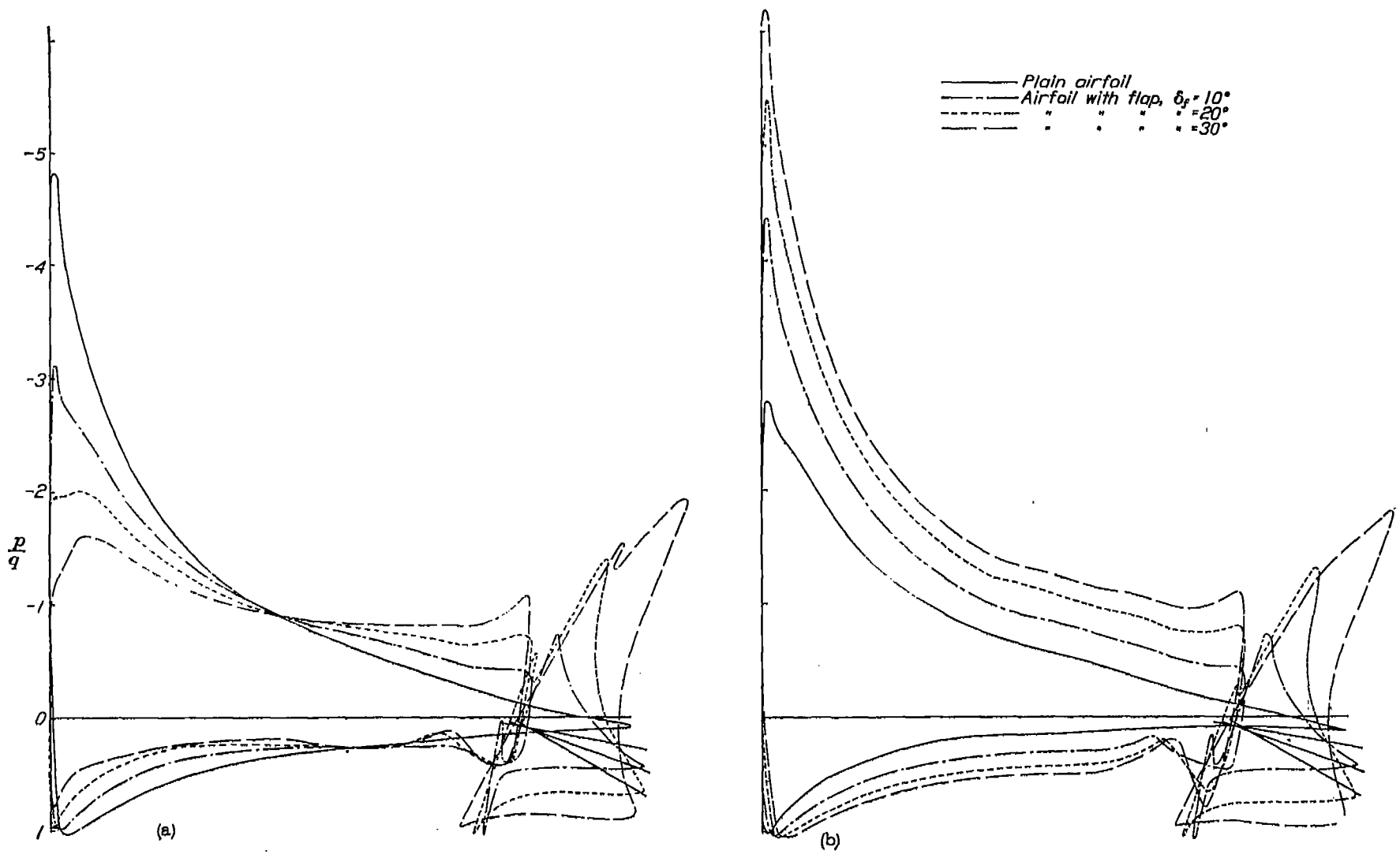
(a) At the same lift, c_{l\alpha} = 1.31 . (b) At the same angle of attack, \alpha_0 = 8^\circ . FIGURE 25.—Comparison of the pressure distribution on an N. A. C. A. 23012 airfoil and a 0.2566c_w slotted flap with that on the plain airfoil.
