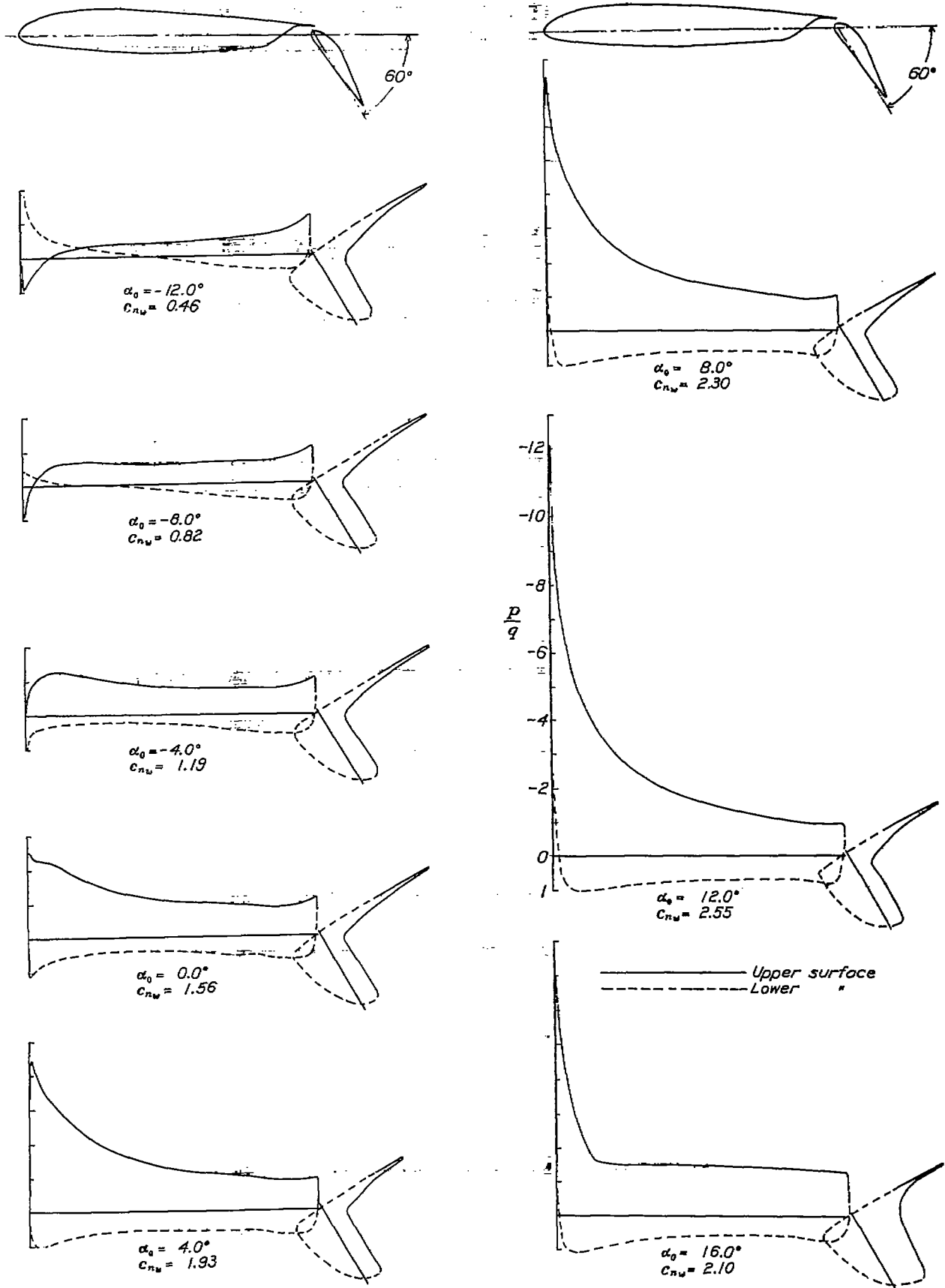
FIGURE 9.—Pressure distribution on the N. A. C. A. 23012 airfoil with a 0.256c slot flap, at various angles of attack. Flap set at 60°.
