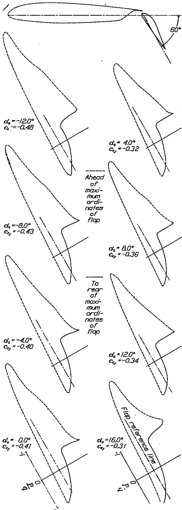
FIGURE 15.—Chord pressure distribution on a 0.2566c slotted flap mounted on the N. A. C. A. 23012 airfoil. Flap set at 60°.
