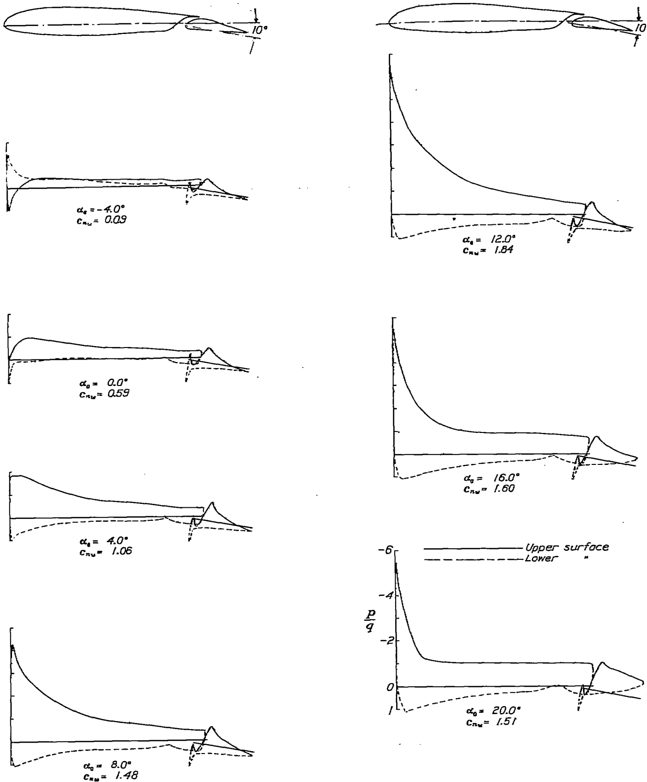
FIGURE 4.—Pressure distribution on the N. A. C. A. 23012 airfoil with a 0.256 c_w slotted flap, at various angles of attack. Flap set at 10°.
