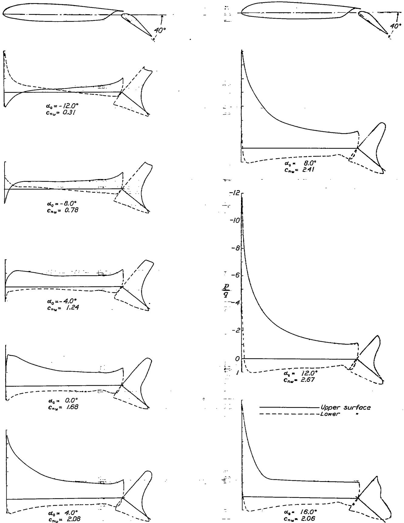
FIGURE 7.—Pressure distribution on the N. A. C. A. 23012 airfoil with a 0.2566c slotted flap, at various angles of attack. Flap set at 40°.
