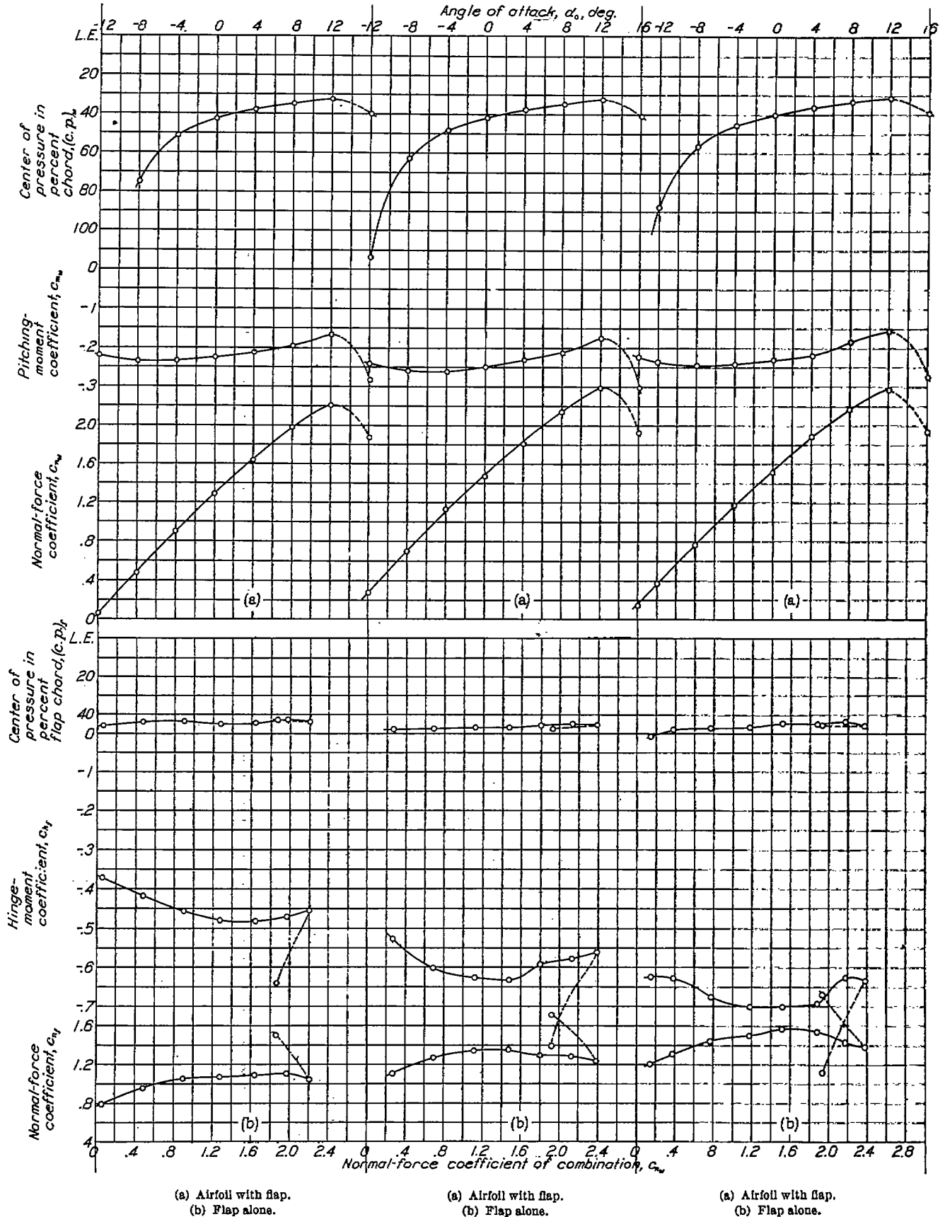
FIGURE 40.—Section characteristics of the N. A. C. A. 23012 airfoil with a 0.20c_w plain flap set at 45^\circ .
