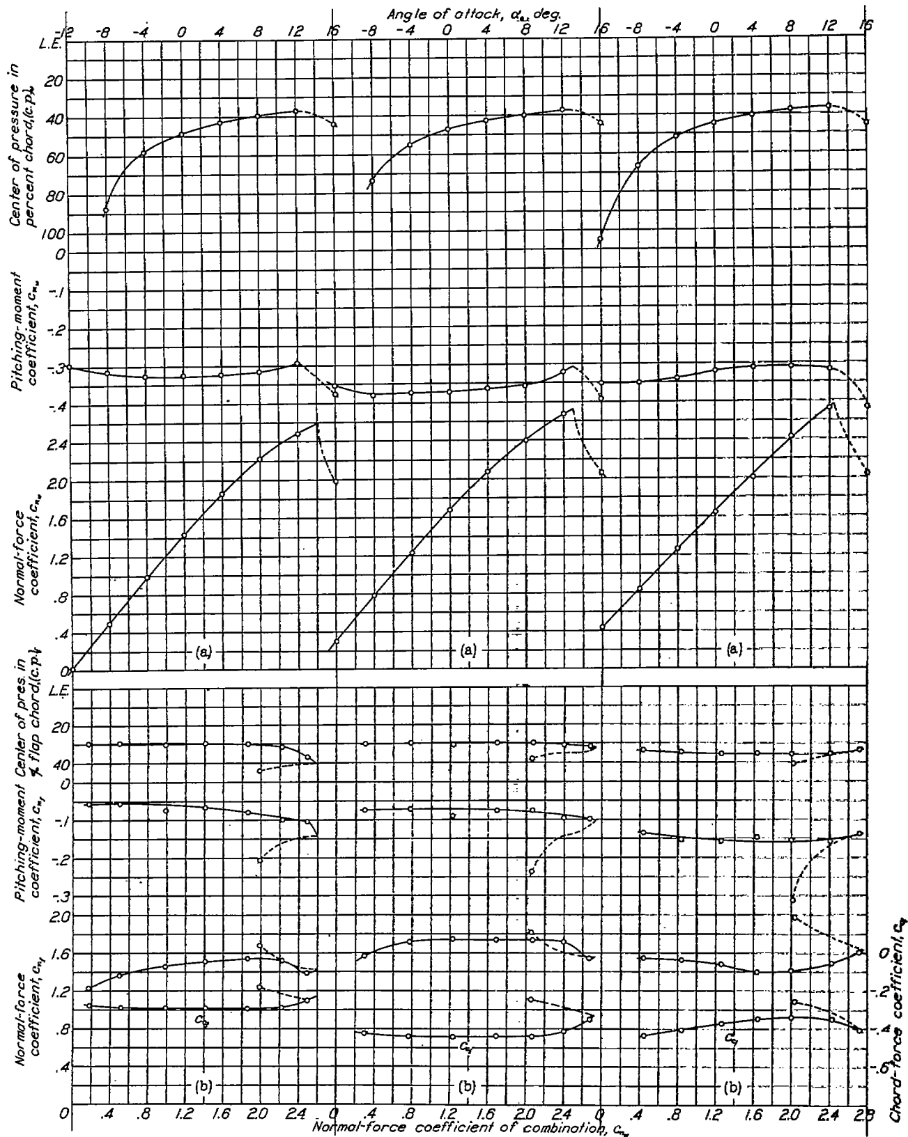
(a) Airfoil with flap. (b) Flap alone.
