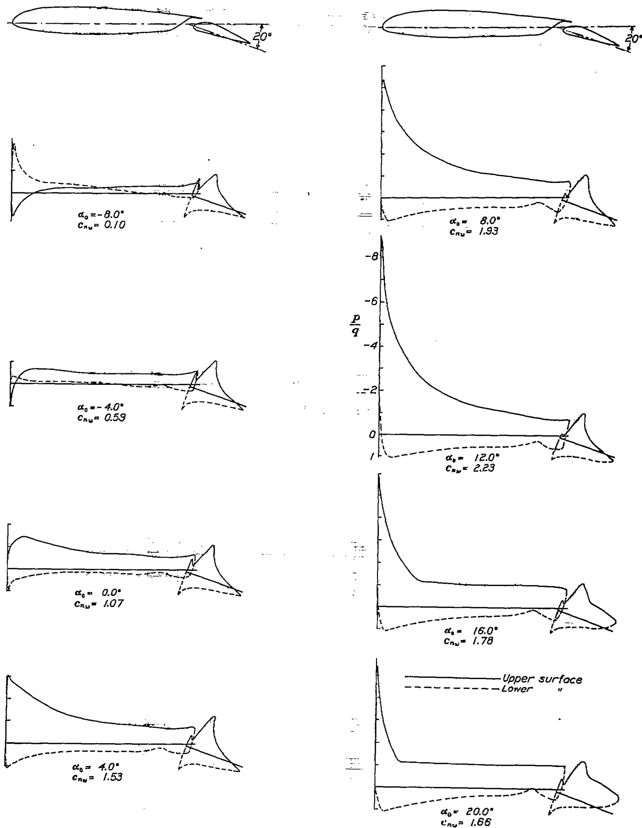
FIGURE 5.—Pressure distribution on the N. A. C. A. 23012 airfoil with a 0.256c w slotted flap, at various angles of attack. Flap set at 20°.
