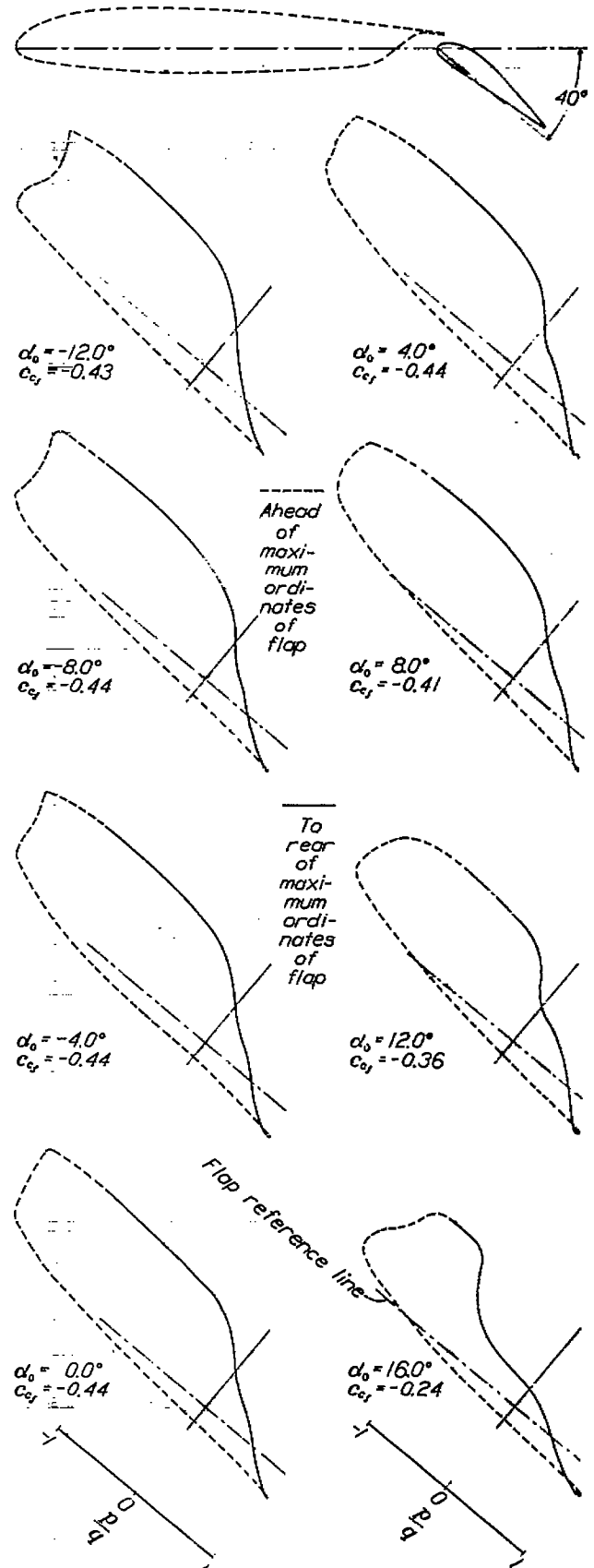
FIGURE 13.—Chord pressure distribution on a 0.256c s slotted flap mounted on the N. A. C. A. 23012 airfoil. Flap set at 40°.
