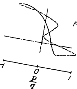
FIGURE 10.—Chord pressure distribution on a 0.2566c s slotted flap mounted on the N. A. C. A. 23012 airfoil. Flap set at 10°.
