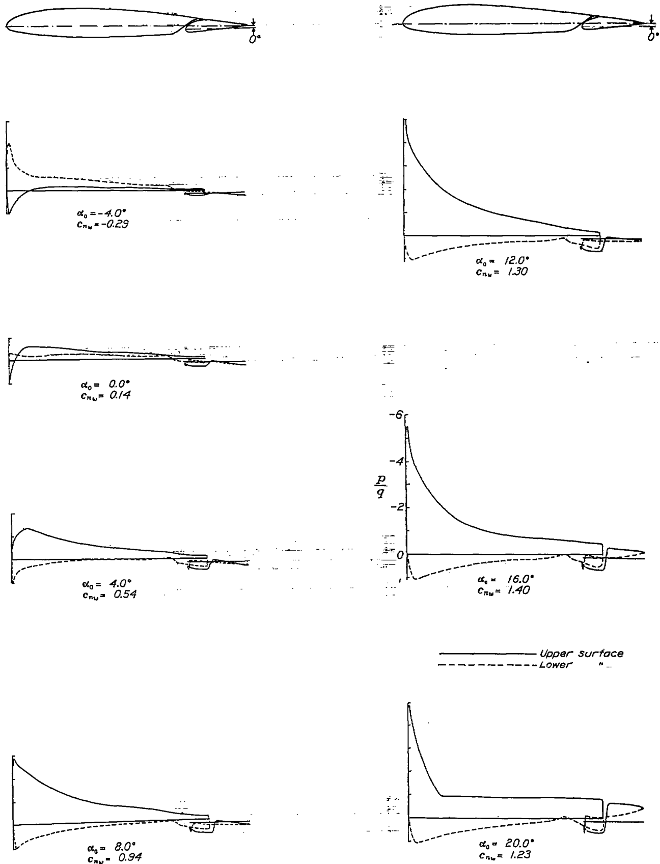
FIGURE 3.—Pressure distribution on the N. A. O. A. 23012 airfoil with a 0.256c w slotted flap, at various angles of attack. Flap set at 0°.
