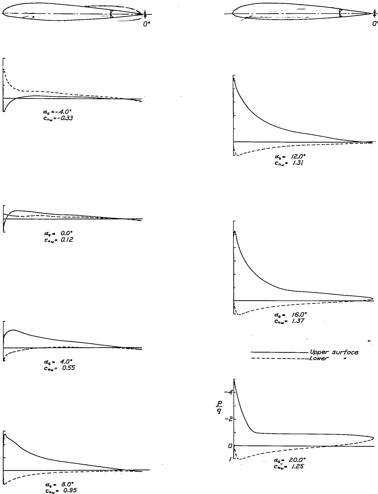
FIGURE 19.—Pressure distribution on the N. A. C. A. 23012 airfoil with a 0.20c u plain flap, at various angles of attack. Flap set at 0°.
