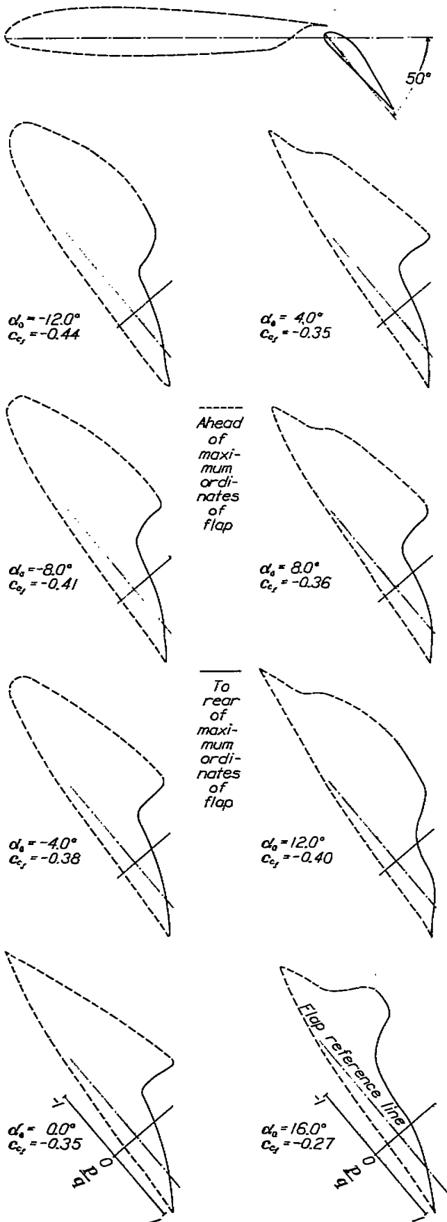
FIGURE 14.—Chord pressure distribution on a 0.2566c slotted flap mounted on the N. A. C. A. 23012 airfoil. Flap set at 50°.
