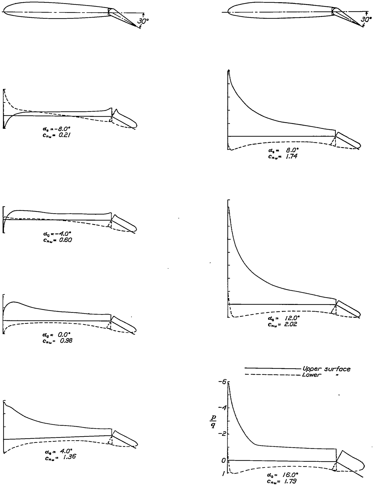
FIGURE 21.—Pressure distribution on the N. A. C. A. 23012 airfoil with a 0.20c plain flap, at various angles of attack. Flap set at 30°.
