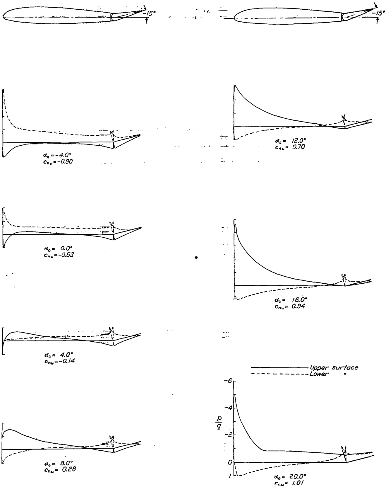
FIGURE 18.—Pressure distribution on the N. A. C. A. 23012 airfoil with a 0.20c_w plain flap, at various angles of attack. Flap set at -15^\circ .
