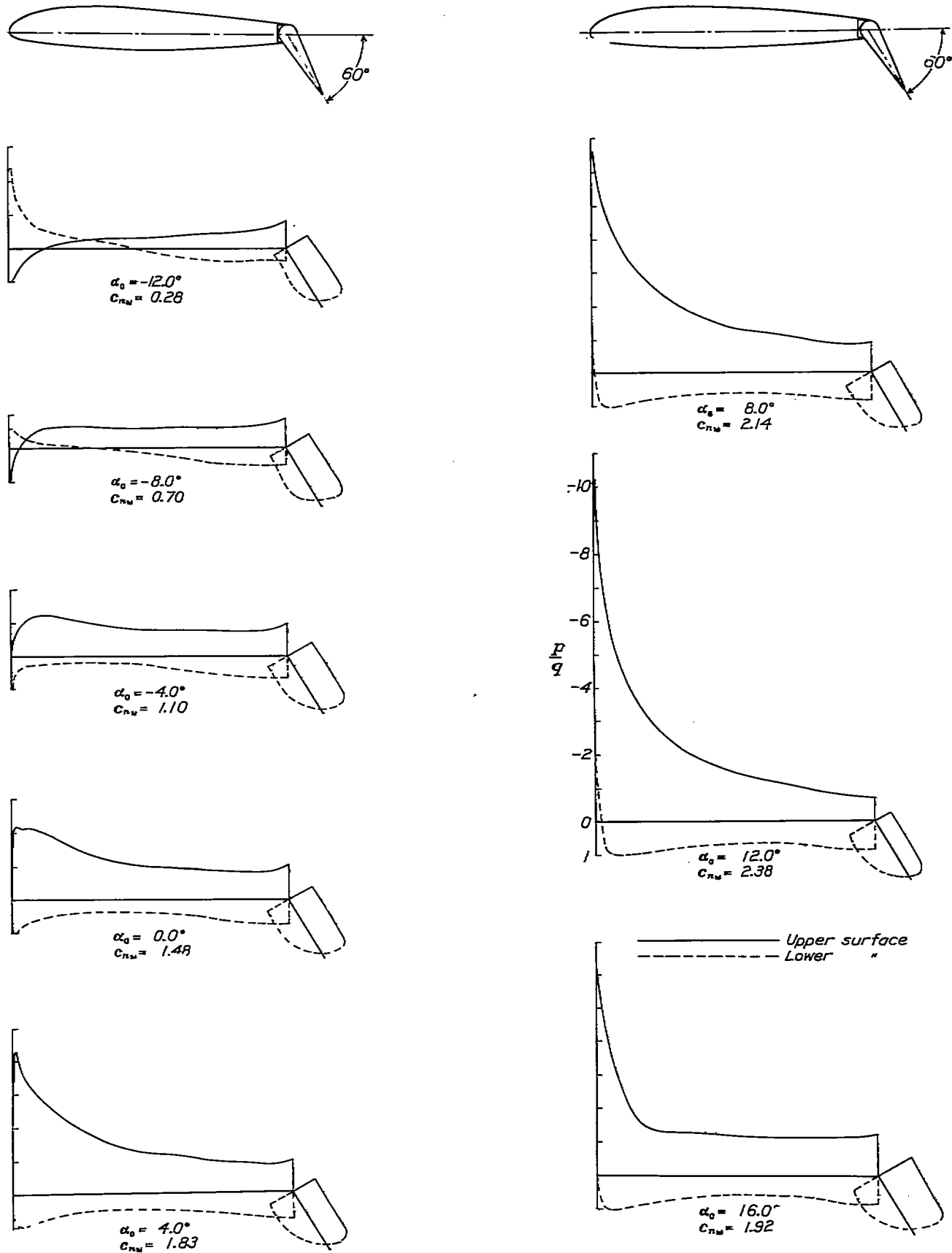
FIGURE 23.—Pressure distribution on the N. A. C. A. 23012 airfoil with a 20% plain flap, at various angles of attack. Flap set at 60°.
