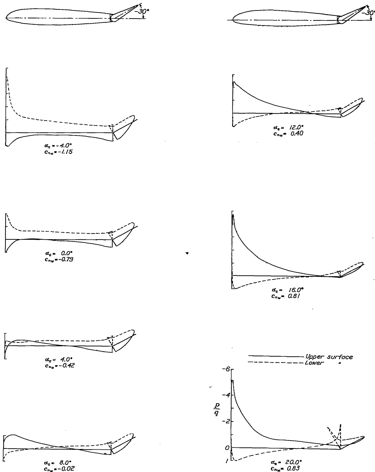
FIGURE 17.—Pressure distribution on the N. A. C. A. 23012 airfoil with a 0.20c_u plain flap, at various angles of attack. Flap set at -30^\circ .
