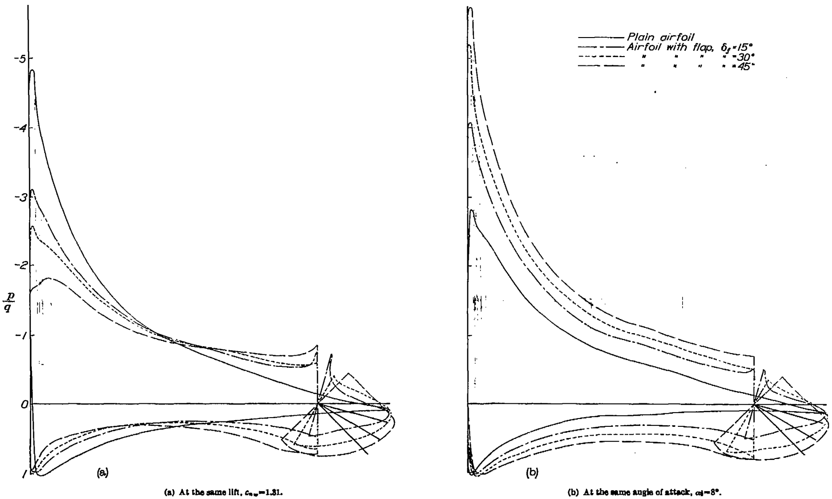
FIGURE 26.—Comparison of the pressure distribution on an N. A. C. A. 23012 airfoil and a 0.20c plain flap with that on the plain airfoil.
