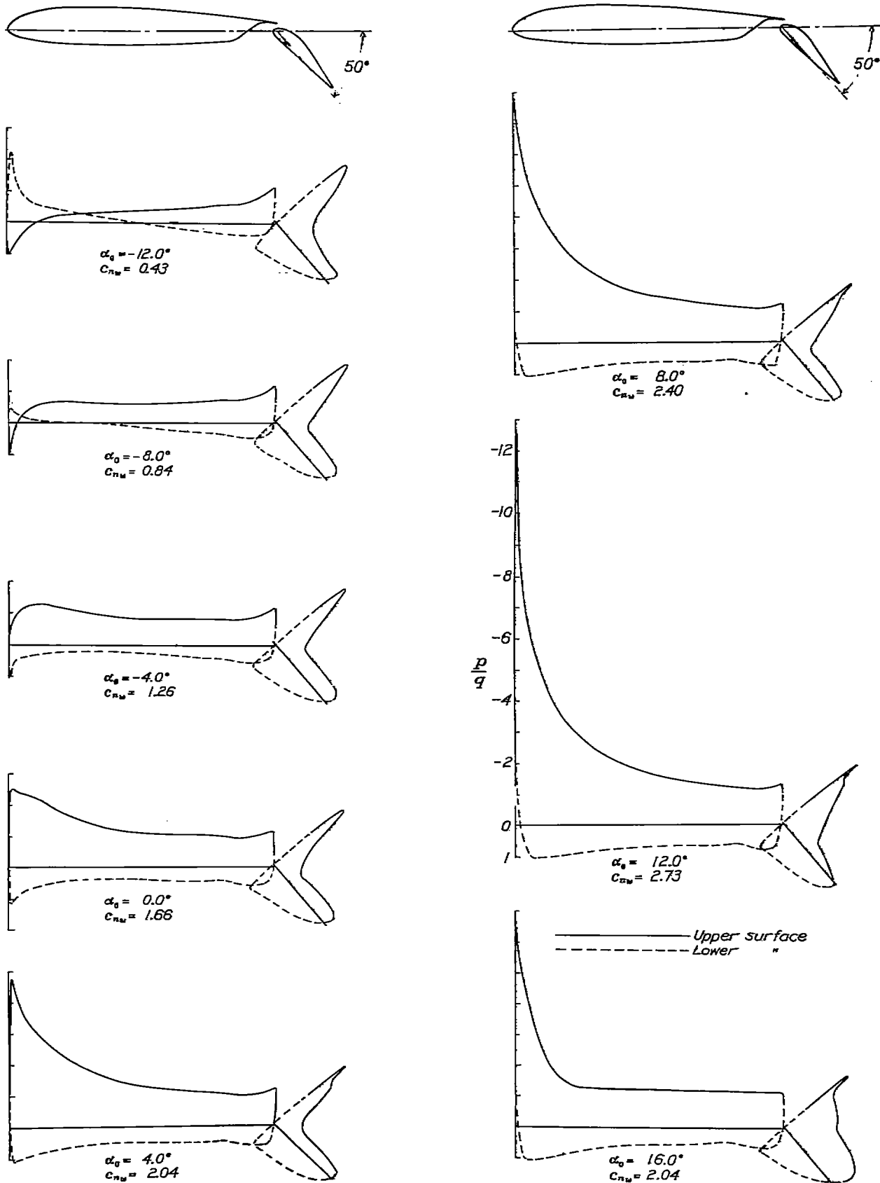
FIGURE 8.—Pressure distribution on the N. A. C. A. 23012 airfoil with a 0.2566c m slotted flap, at various angles of attack. Flap set at 50°.
