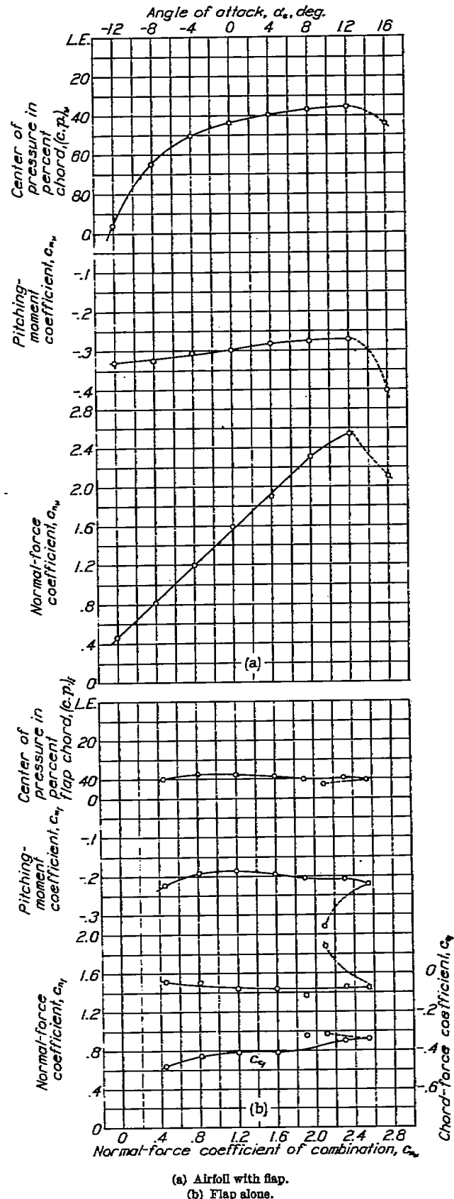
FIGURE 33.—Section characteristics of the N. A. C. A. 23012 airfoil with a 0.2566c slotted flap set at 60^\circ .
