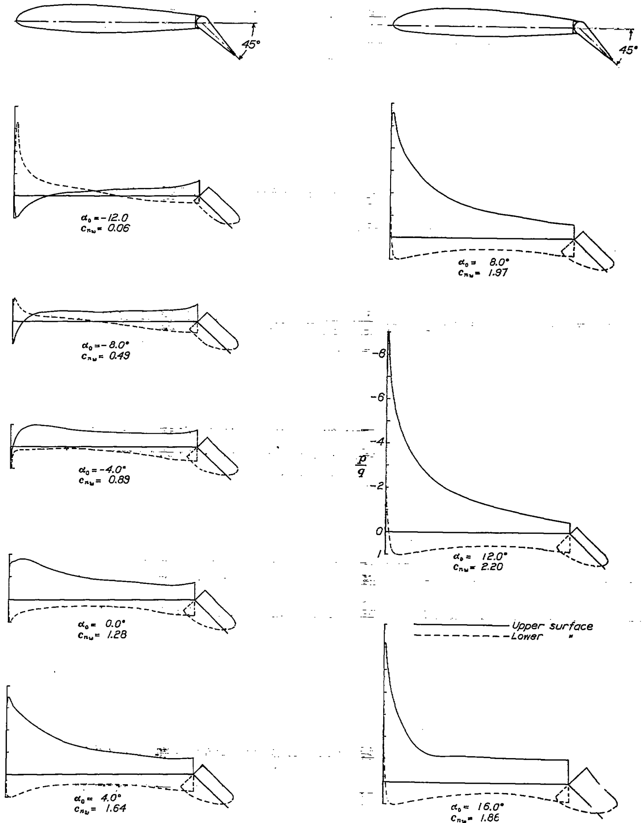
FIGURE 22.—Pressure distribution on the N. A. C. A. 23012 airfoil with a 0.20 c_w plain flap, at various angles of attack. Flap set at 45°.
