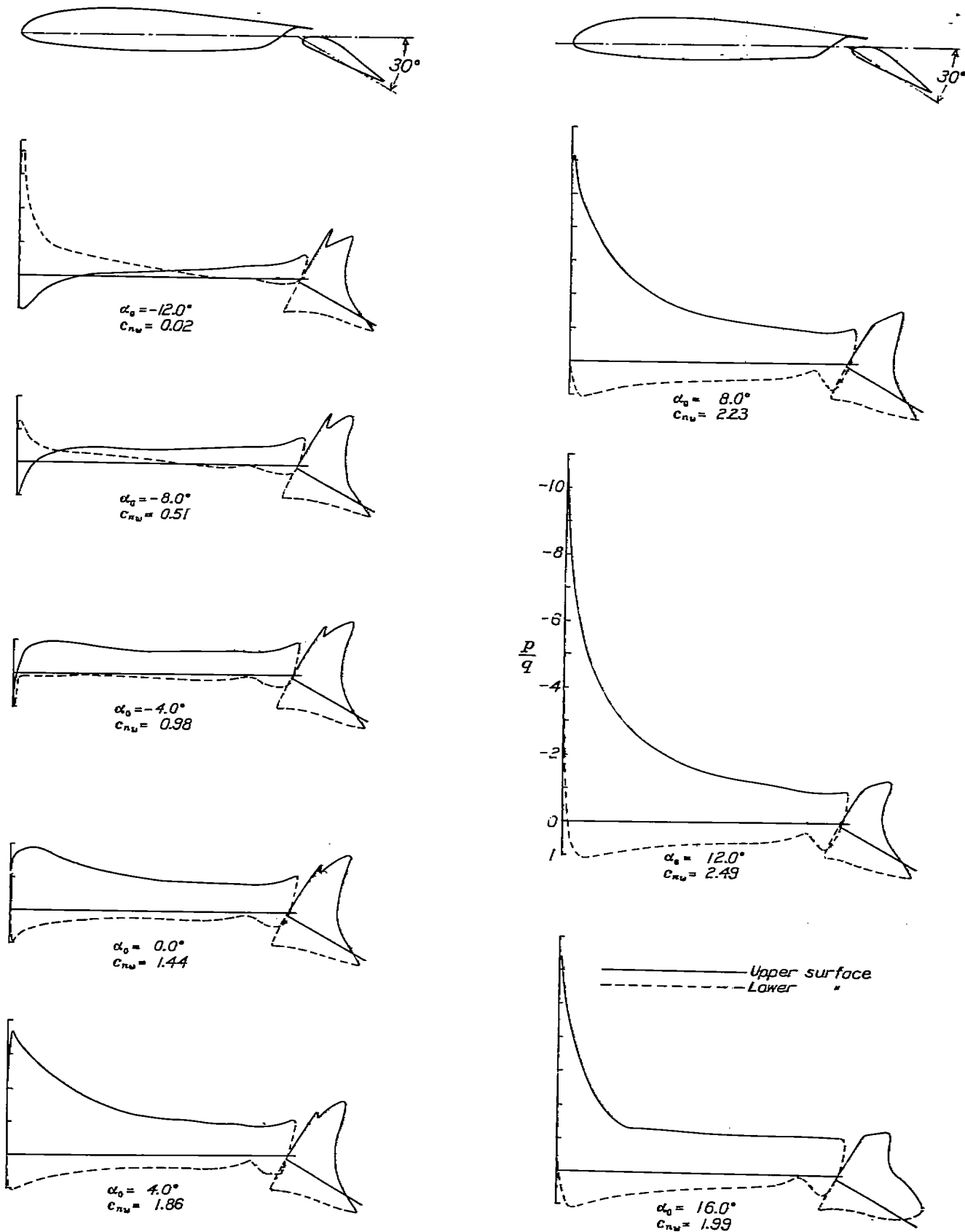
FIGURE 6.—Pressure distribution on the N. A. C. A. 23012 airfoil with a 0.256 c_w slotted flap, at various angles of attack. Flap set at 30°.
