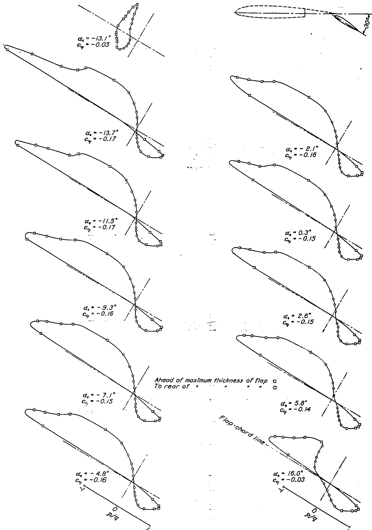
FIGURE 13.—Chord pressure distribution on the 0.30c N. A. C. A. 23012 Fowler flap mounted on the N. A. C. A. 23013 airfoil. Flap deflected 30°.
