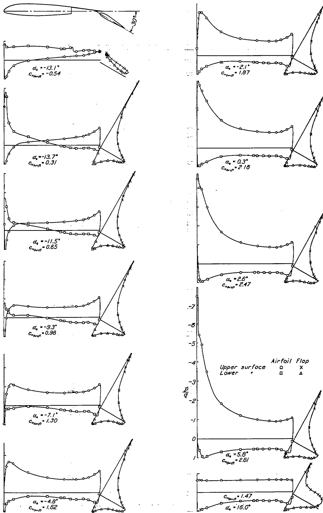
FIGURE 9.—Pressure distribution on the N. A. C. A. 23012 airfoil, with the 0.3c N. A. C. A. 23012 Fowler flap, at various angles of attack. Flap deflected 30°.
