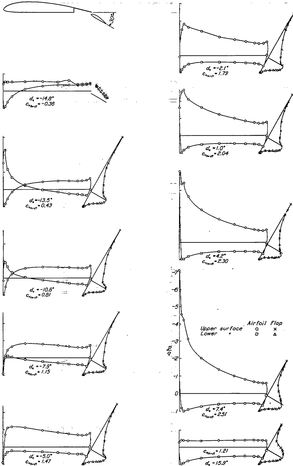
FIGURE 7.—Pressure distribution on the Clark Y airfoil, with the 0.20c Clark Y Fowler flap, at various angles of attack. Flap deflected 30°.
