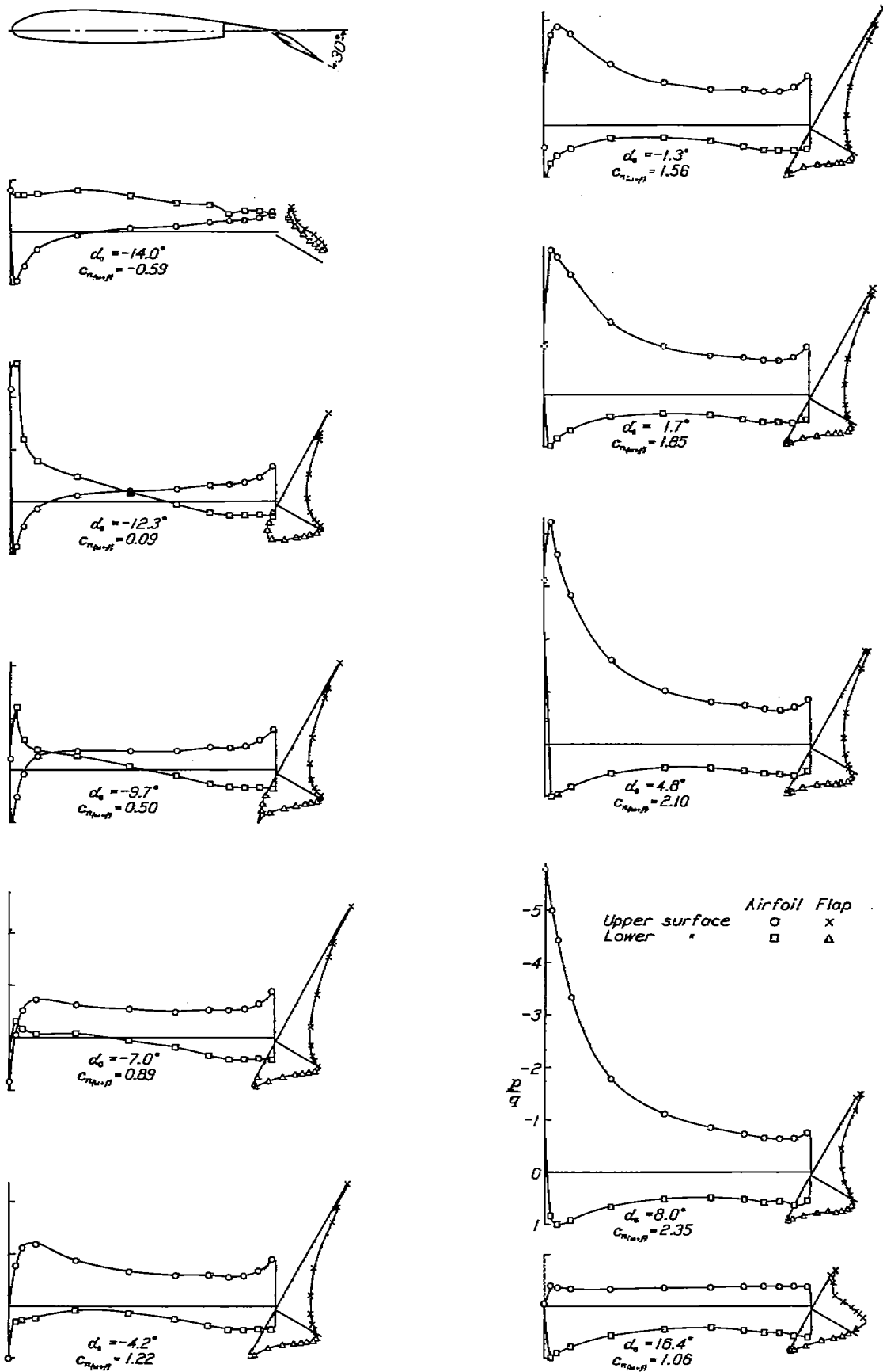
FIGURE 8.—Pressure distribution on the N. A. C. A. 23012 airfoil, with the 0.20 N. A. C. A. 23012 Fowler flap, at various angles of attack. Flap deflected 30°. 189778—39—13
