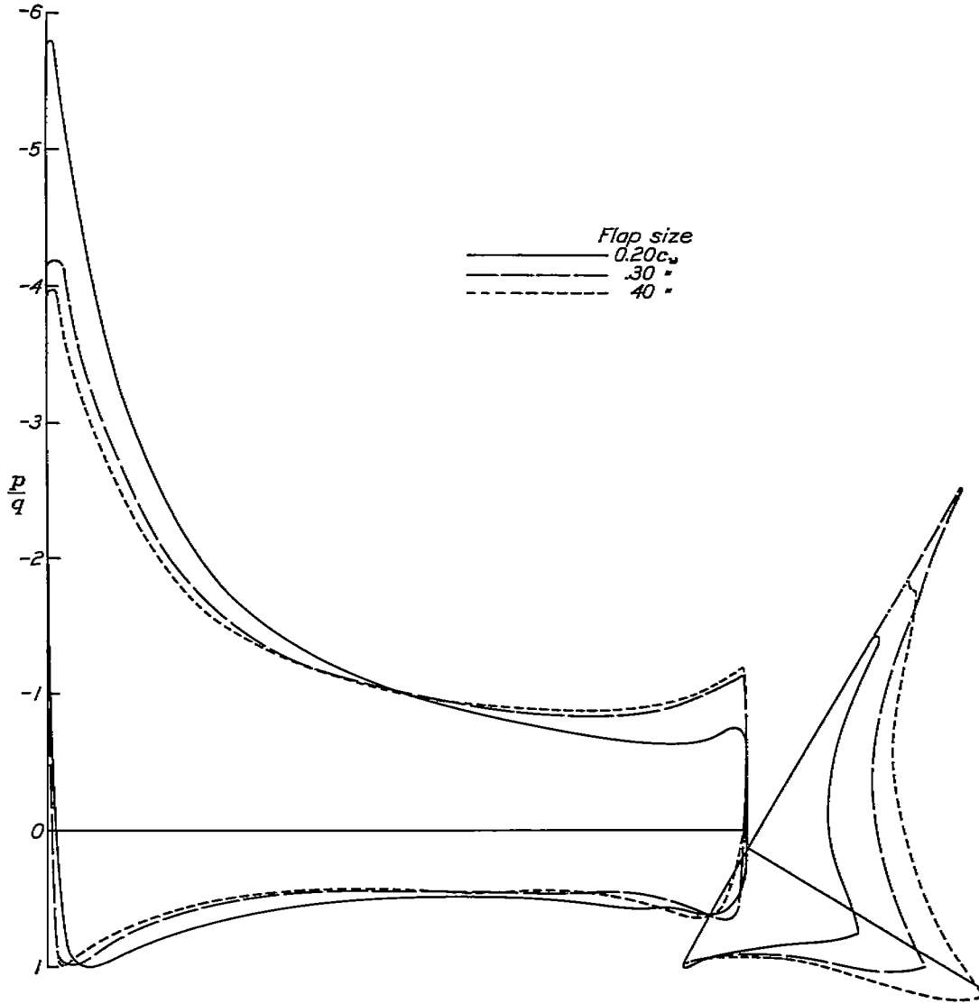
FIGURE 12.—Comparison of the pressure distribution, at the same lift, on the N. A. C. A. 23012 airfoil with the 0.20 c_w , the 0.30 c_w , and the 0.40 c_w N. A. C. A. 23012 Fowler flaps. c_{n(w+f)} = 2.35 .
