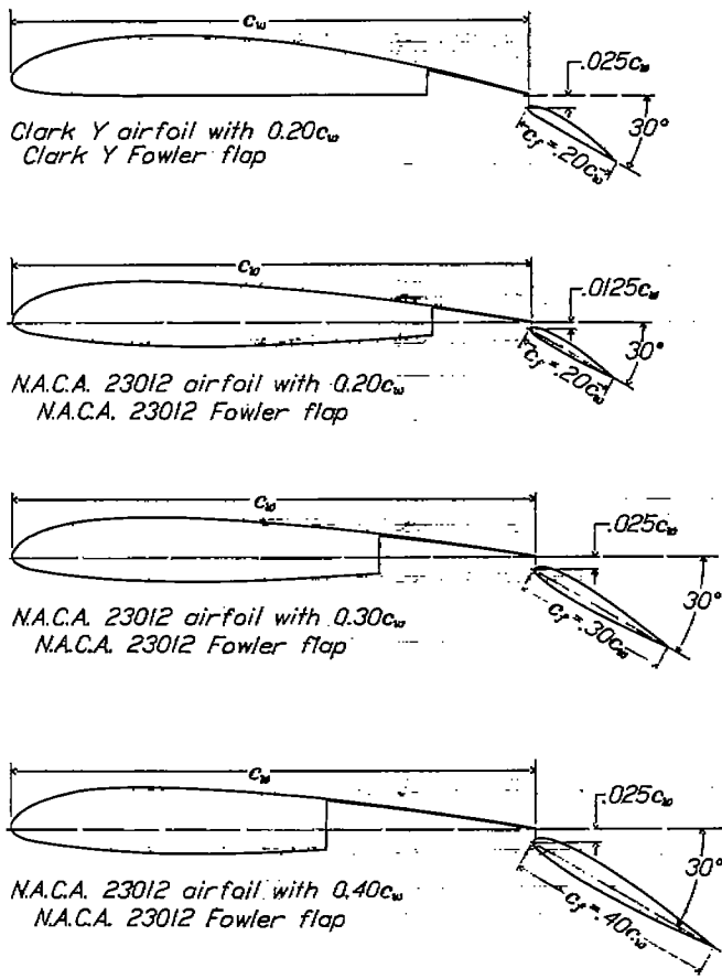
FIGURE 1.—Sections of airfoil and flap combinations tested.
