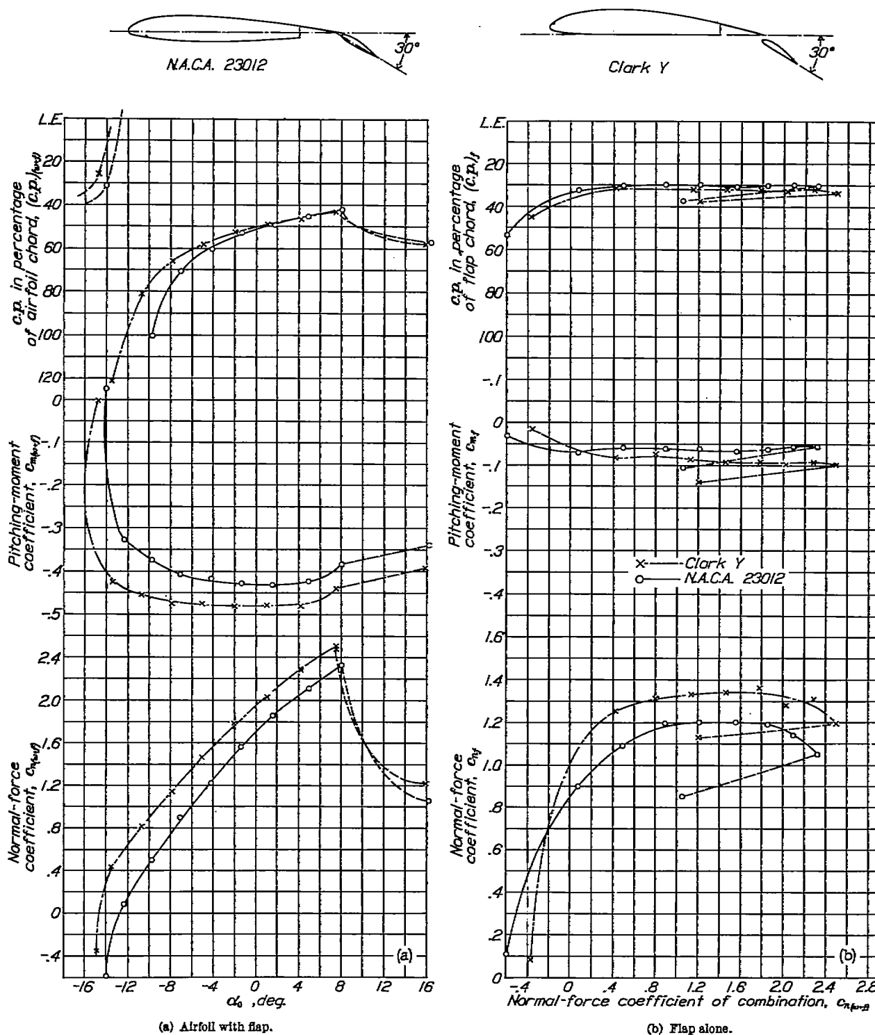
FIGURE 16.—Section characteristics of the N. A. C. A. 23012 airfoil with the 0.20c u N. A. C. A. 23012 Fowler flap and of the Clark Y airfoil with the 0.20c u Clark Y Fowler flap. Flaps deflected 30°.
