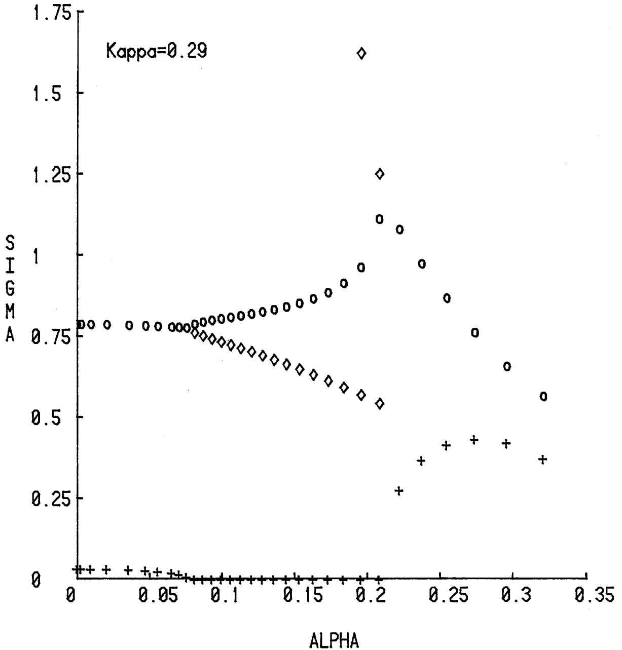
Figure 60. Calculated non-dimensional eigenvalues ( \sigma \cdot l^2 / \Gamma ) from the linear stability analysis.
