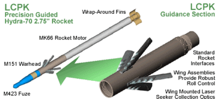
Fig. BAE Systems LCPK.
